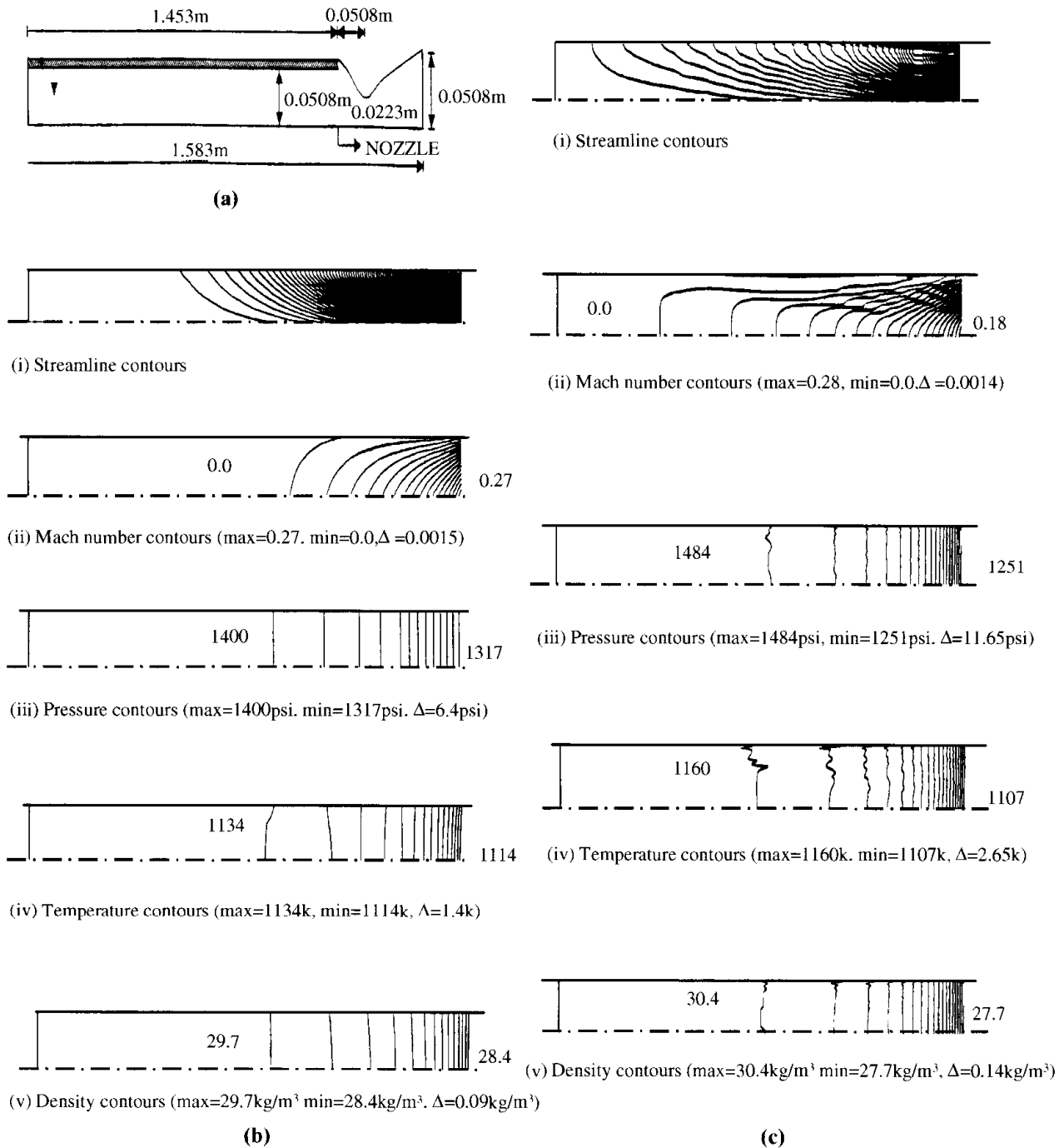
Figure 23.5.3.1 State flowfield for side-burning rocket motor, burning surface boundary conditions: \rho = 29.7 \text{ kg/m}^3 , V = 1.22 \text{ m/s} , T = 1134 \text{ K} , P = 1400 \text{ psi} , Mach no. = 0.0018, laminar calculations [Yoon and Chung, 1994]. (a) Geometry. (b) 0% disturbance. (c) 6% disturbance.
