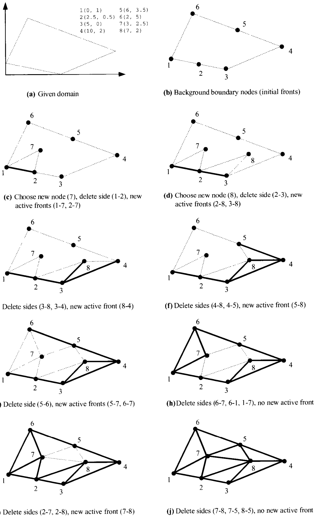
Figure 18.2.2 General procedure for advancing front methods (AFM) for simply connected domain, boundaries of dash areas represent active advancing fronts. Deleted lines constitute the generated mesh.
