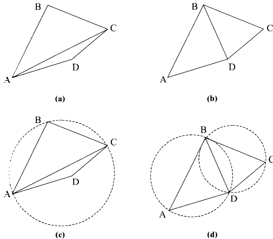
Figure 18.1.2 A triangulation must satisfy the in-circle criterion that no point of the set P_i is interior to the circumcircle of any triangle T(P_i) . (a) Undesirable triangulation, maximum-minimum criterion is not satisfied. (b) Desirable triangulation, maximum-minimum criterion is satisfied. (c) Unacceptable because the circumcircle ABC includes point D interior to the circumcircle. Similarly, if circumcircle ACD is drawn, then B will be interior to it. (d) Acceptable because no point is interior to the circumcircles (ABD or BCD).
