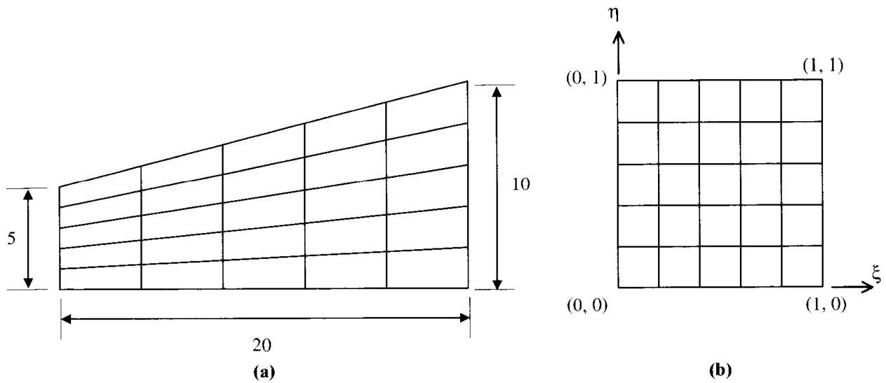
Figure E17.1.1 Physical (trapezoidal) and transformed geometries.
