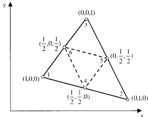
Figure 9.3.4 Natural coordinate triangular element (quadratic variation).
