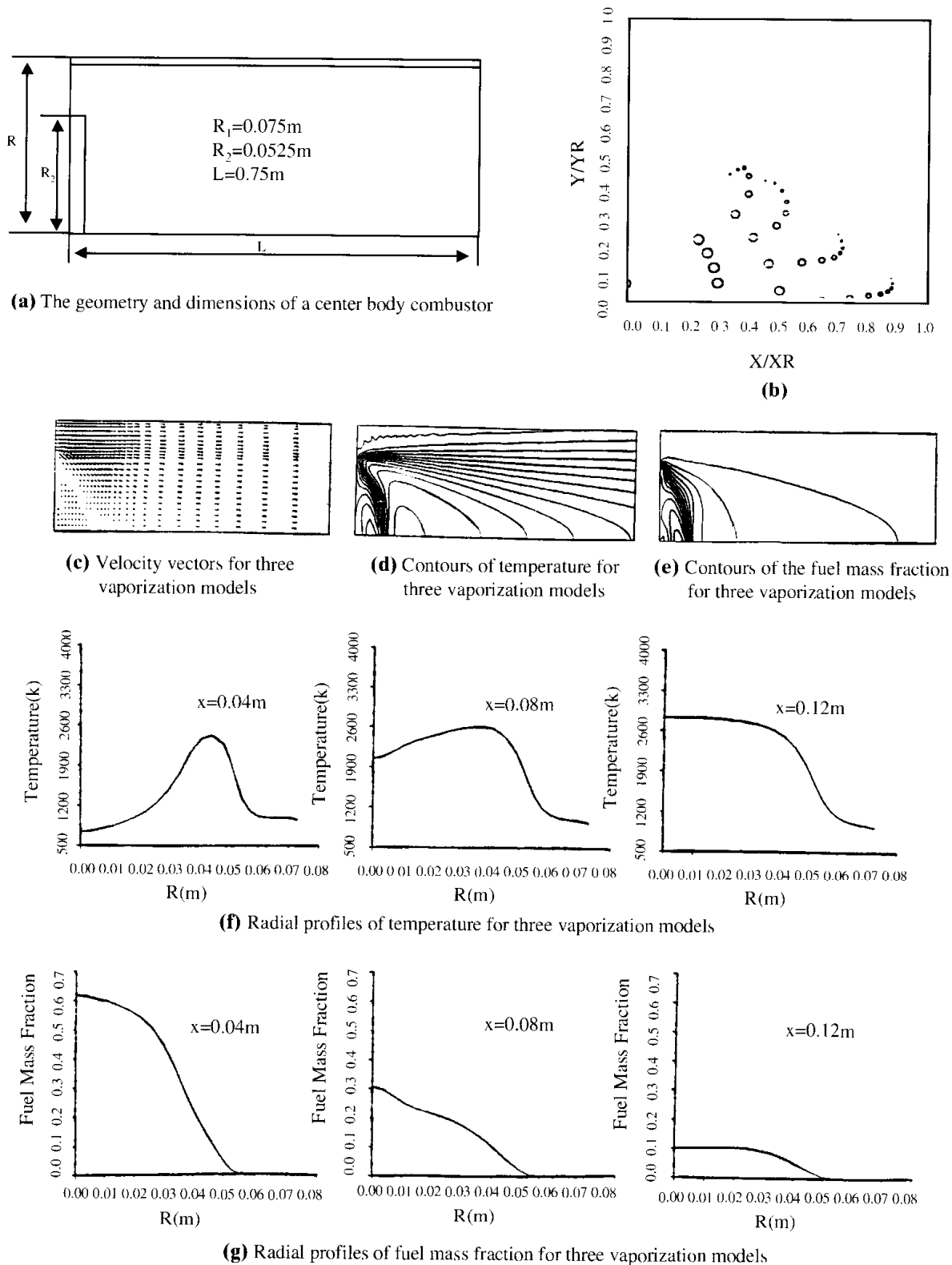
Figure 22.6.5.1 Spray combustion of center body combustor [Kim and Chung, 1990].
