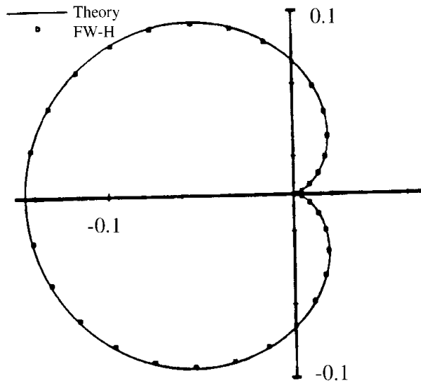
Figure 23.5.2.3 Acoustic pressure squared at r = 50a for line vertex moving around semi-infinite plate with M = 0.01 [Singer et al., 1999].
