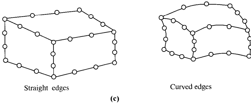
Figure 9.4.5 Hexahedral isoparametric element: (a) linear variation (8 nodes); (b) quadratic variation (20 nodes); (c) cubic variation (32 nodes).
