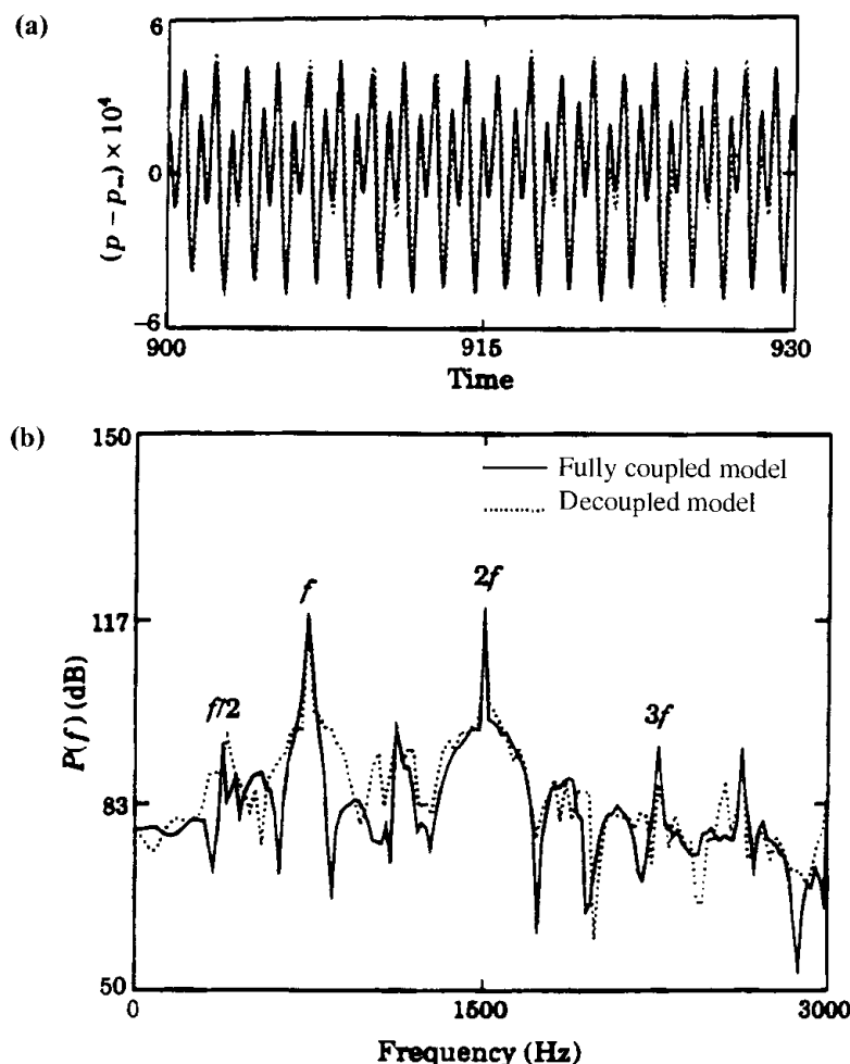
Figure 23.5.1.5 (a) The time history and (b) power spectral density of the transmitted far-field pressure, 203.2 cm from the panel center, excitation amplitude 174 dB (nonlinear) [Frendi et al., 1995]. Reprinted with permission from Academic Press.
