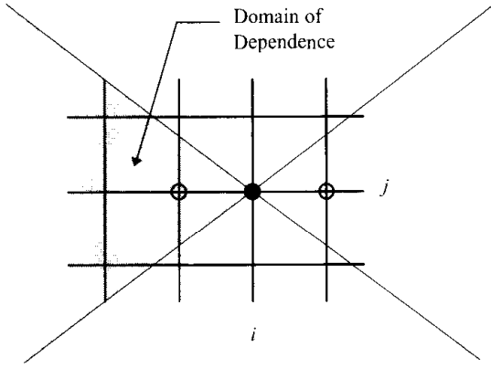
Figure 6.1.1 Region of dependence.
