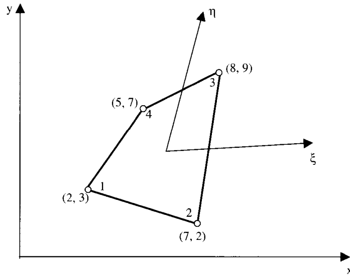
Figure E9.3.2 Geometry for Example 9.3.2.
