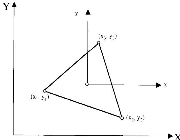
Figure 9.3.1 Cartesian coordinate triangular element.
