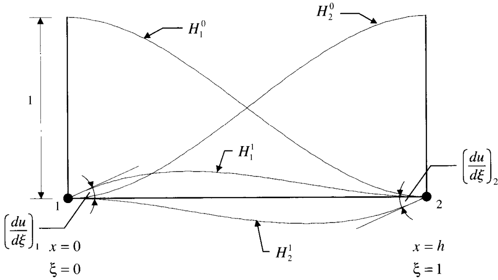
Figure 9.2.3 Hermite interpolation functions.
