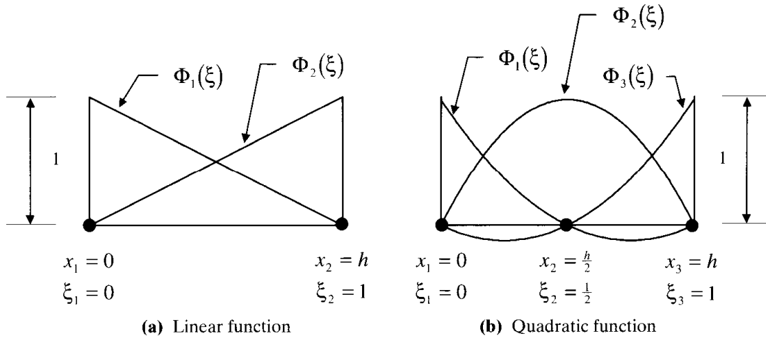
Figure 17.1.1 Lagrange polynomials.
