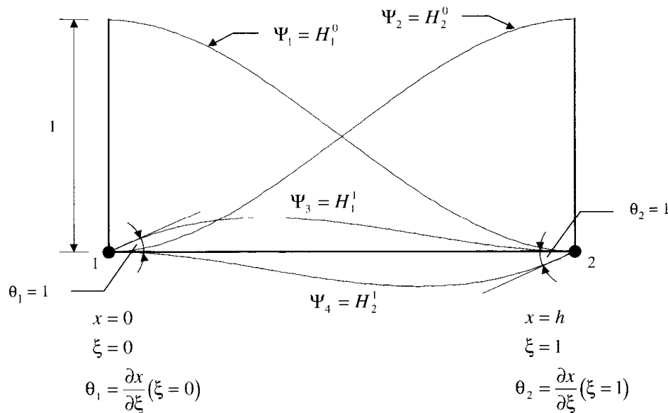
Figure 17.1.2 Hermite polynomial.
