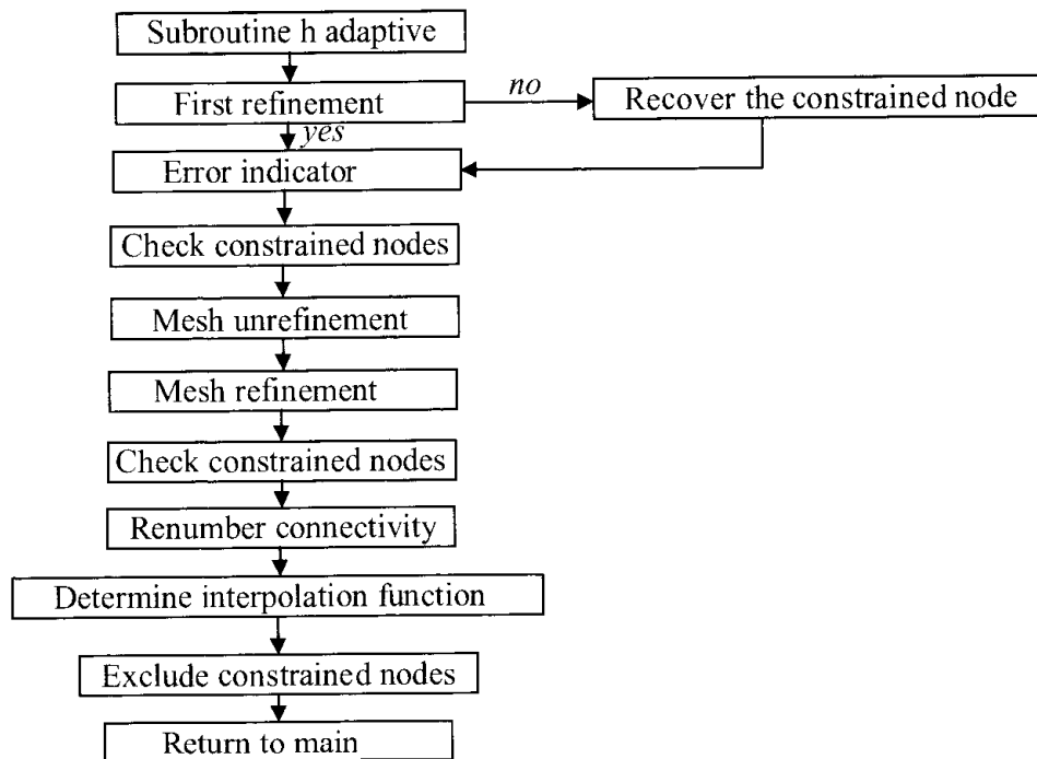
Figure 19.2.2 Flow diagram for mesh refinements.
