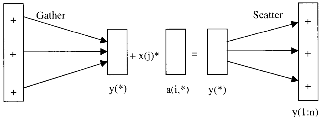
Figure 20.3.4 Column-oriented matrix-by-vector multiplication – Scatter operation.
