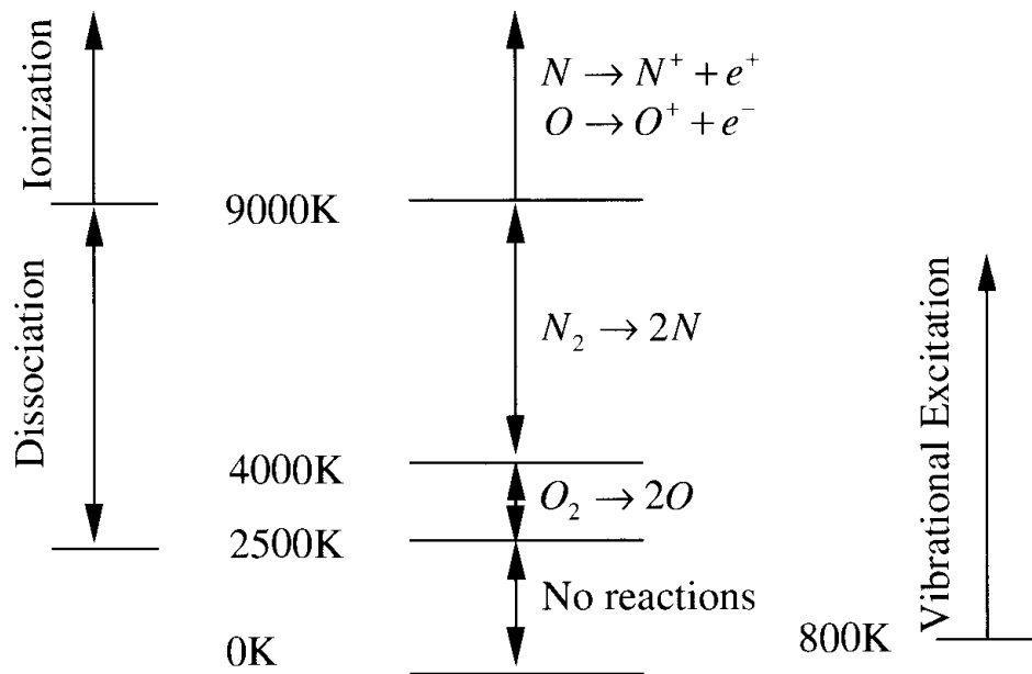
Figure 22.5.2 Ranges of vibrational excitation, dissociation, and ionization for air at 1 atm.
