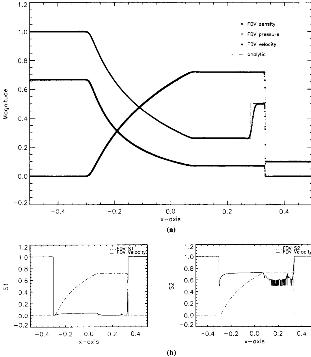
Figure 27.3.4.1 Relativistic shock tube analyzed by the FDV theory, 1,600 nodes, CFL = 0.18, \alpha = 0.001 , and \eta = 0.25 [Richardson, 2000]. (a) Density, pressure, and velocity distributions. (b) Calculate values of convection variation parameters ( s_1 , s_2 ).
