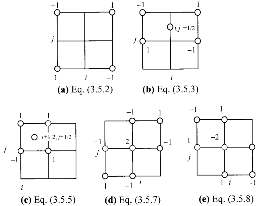
Figure 3.5.1 Mixed derivatives.
