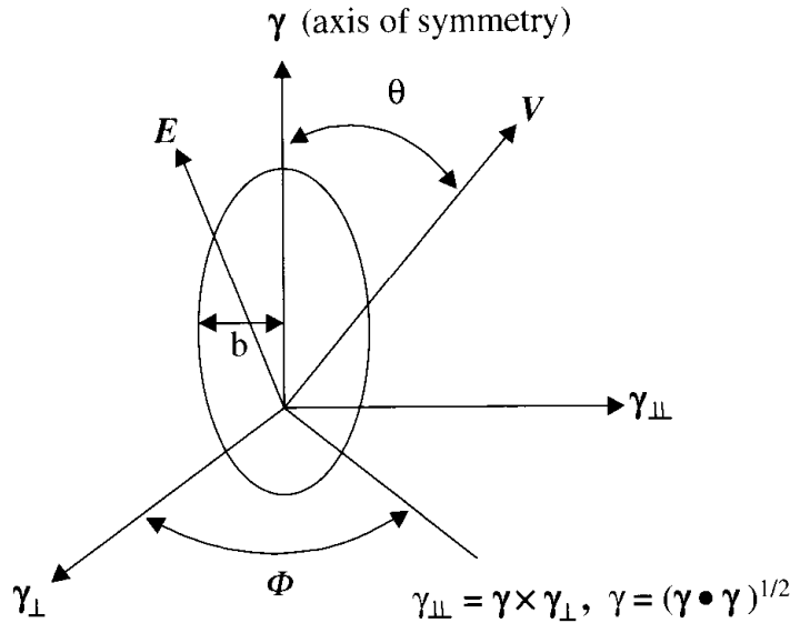
Figure 26.3.2 The surface of an ellipsoid of revolution describes the distribution function in three dimensions. The electric field is shown for the general case in which it is not aligned with the axis of symmetry ( 0 < \gamma < 1 ).
