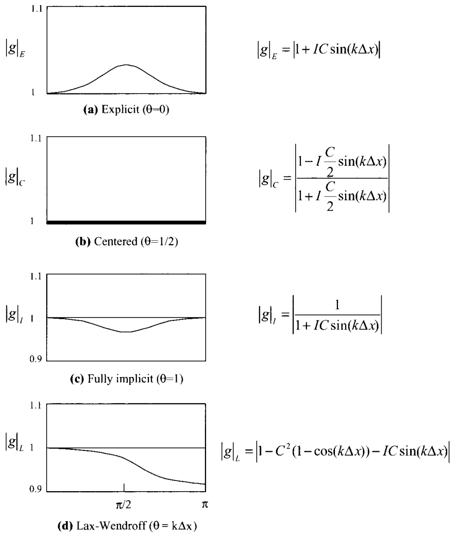
Figure 4.5.3 Amplification factors.
