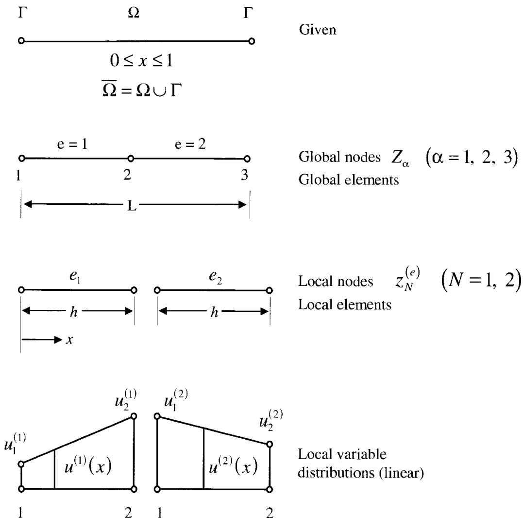
Figure 8.2.1 Finite element approximations.
