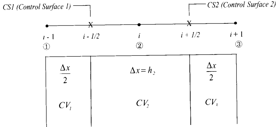
Figure 1.4.1 Finite volume approximations.
