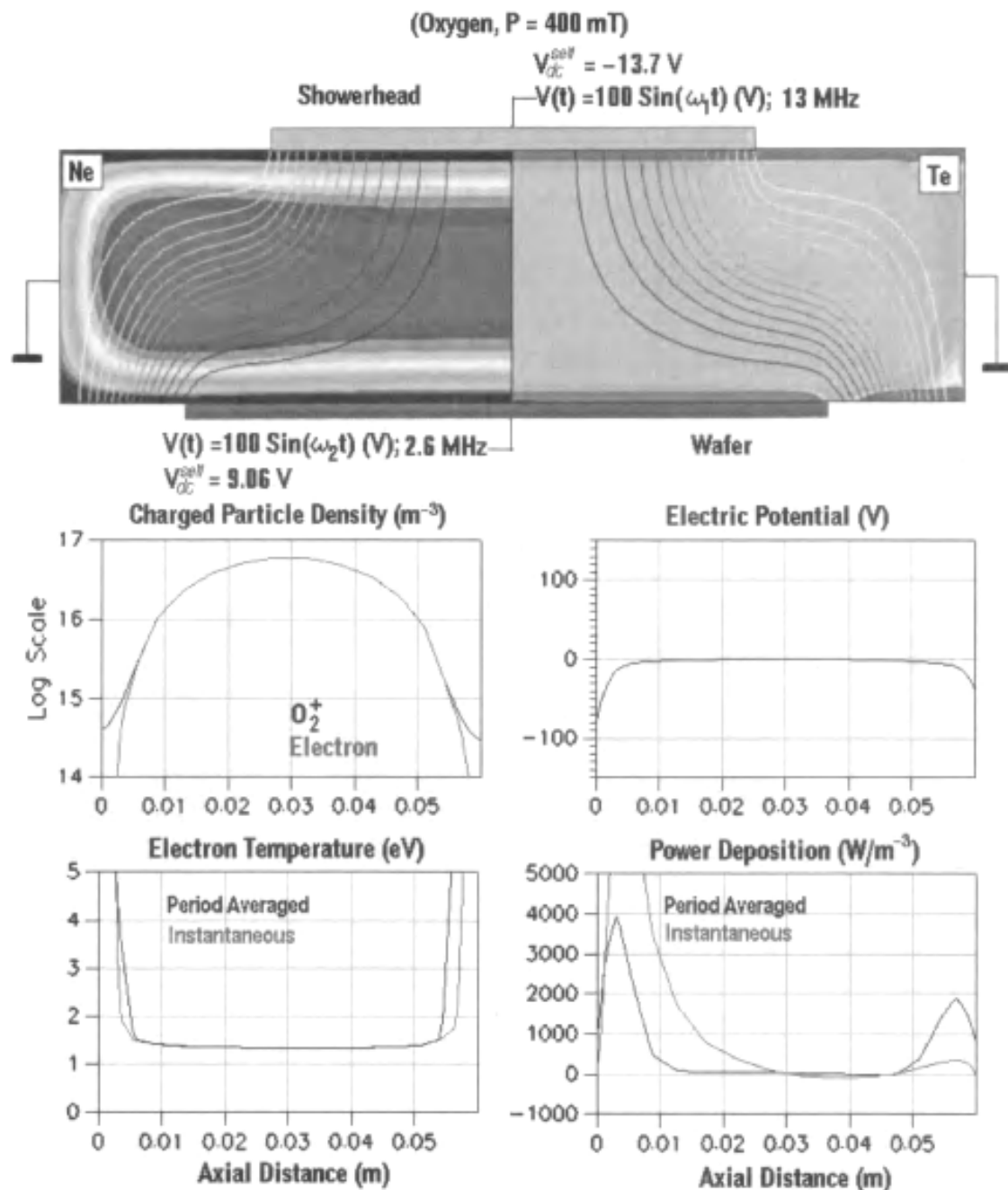
Figure 26.4.2.3 Dual-frequency capacitively coupled plasma [Courtesy of CFDRC].
