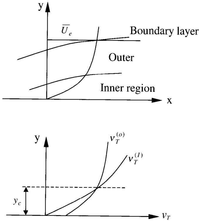
Figure 21.3.2 One-equation model [Cebeci-Smith, 1974; Baldwin-Lomax, 1978].
