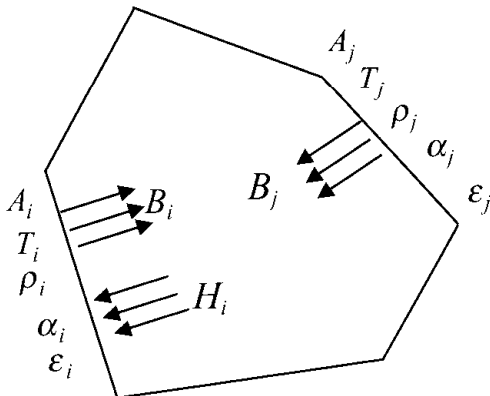
Figure 24.2.1 Enclosure filled with nonparticipating medium.
