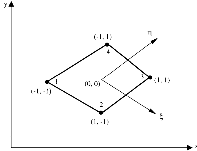
Figure 9.3.10 Quadrilateral isoparametric element (linear variation).
