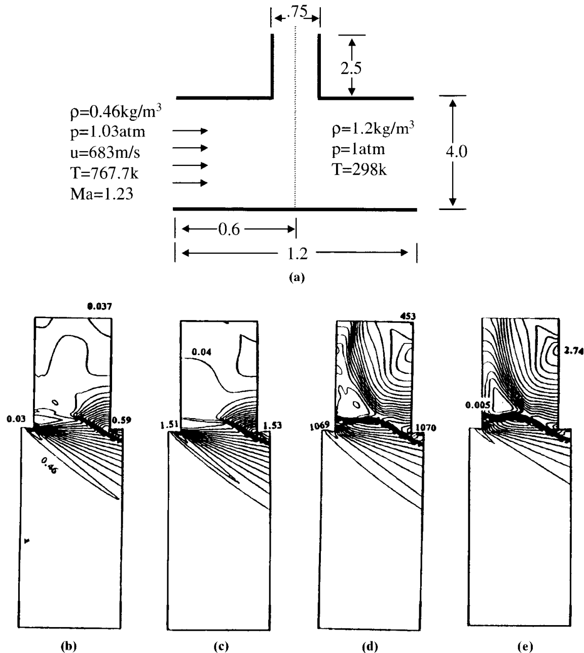
Figure 23.5.1.13 Geometry and flowfields in a perforated muzzle break at steady-state. (a) Geometry and initial boundary conditions. (b) Density. (c) Pressure. (d) Temperature. (e) Mach number.
