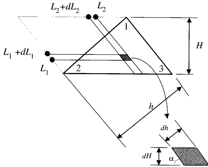
Figure 9.3.7 Geometry for area coordinate integration.
