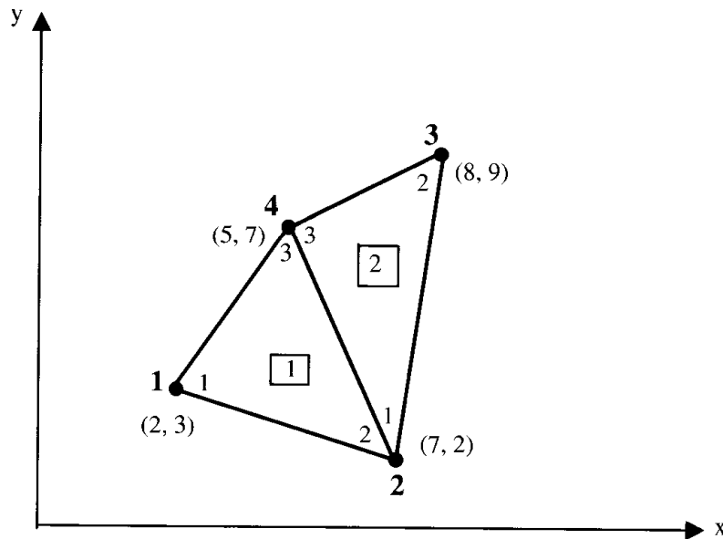
Figure E10.1.1 Assembly of two triangular elements.
