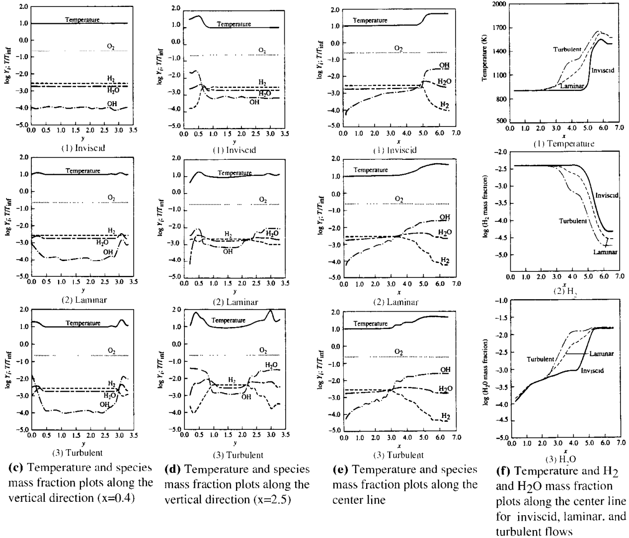
Figure 22.6.2.2 Turbulent ( k-\epsilon model) scramjet flame holder combustion, comparison with inviscid and laminar flames [Yoon, 1992].
