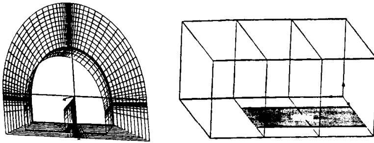
Figure 19.1.4 ONENA M6 wing multiblock [Kim and Thompson, 1990].
