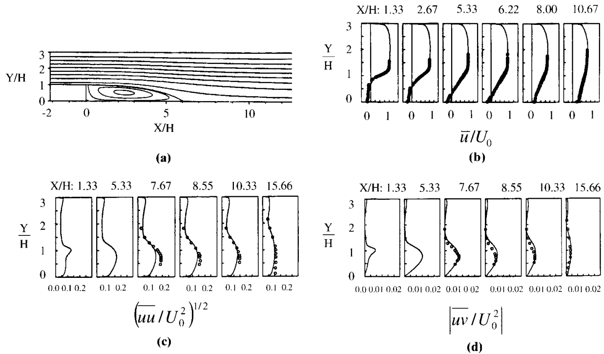
Figure 21.7.1.2 Results with the standard K-ε two-layer model [Thangam and Speziale 1988], compared with Kim et al. [1980]. (a) Contours of mean streamlines. (b) Mean velocity profiles at selected locations, compared with experiments [Kim et al., 1980]. (c) Turbulence intensity profiles. (d) Turbulence shear stress profiles.
