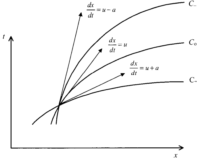
Figure 6.2.2 Characteristic lines for one-dimensional flow.
