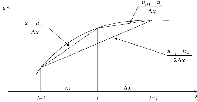
Figure 1.2.1 Finite difference approximations.
