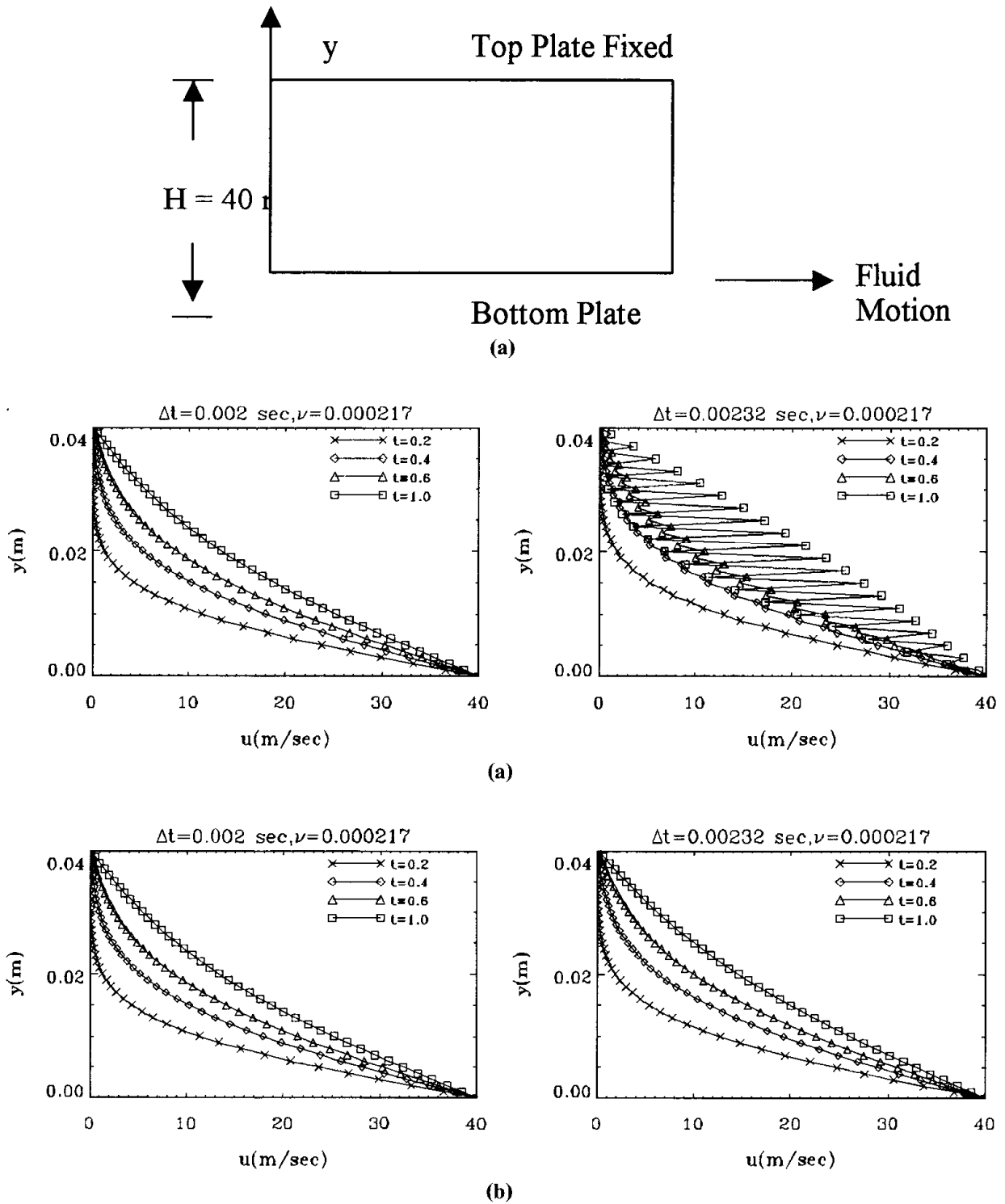
Figure 4.7.2.1 Couette flow. (a-top) Couette flow geometry. (a-bottom) Velocity profiles for FTCS explicit method (40 elements). (b) Velocity profiles for Crank-Nicolson method (40 elements).
