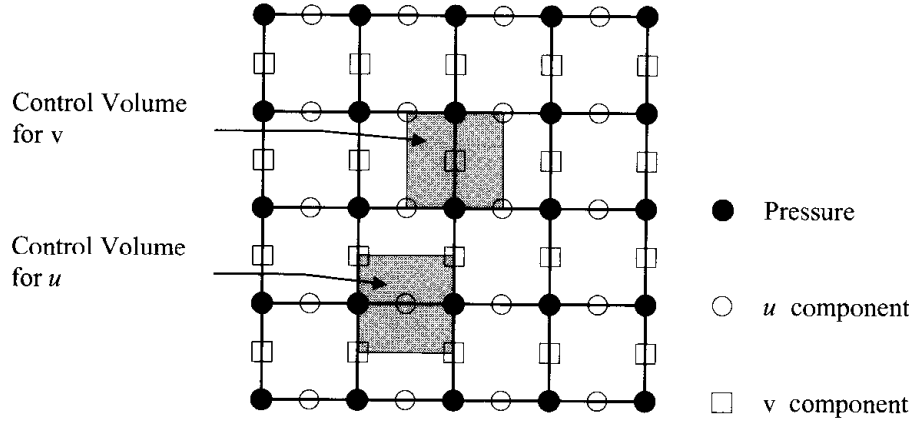
Figure 5.3.1 Computational domain for staggered grid.
