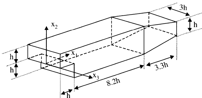
Figure 21.7.2.1 Backward-facing step 3-D geometry for LES analysis [Fureby, 1999].
