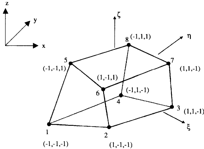
Figure 7.3.4 Three-dimensional control volume with hexahedral isoparametric coordinates.
