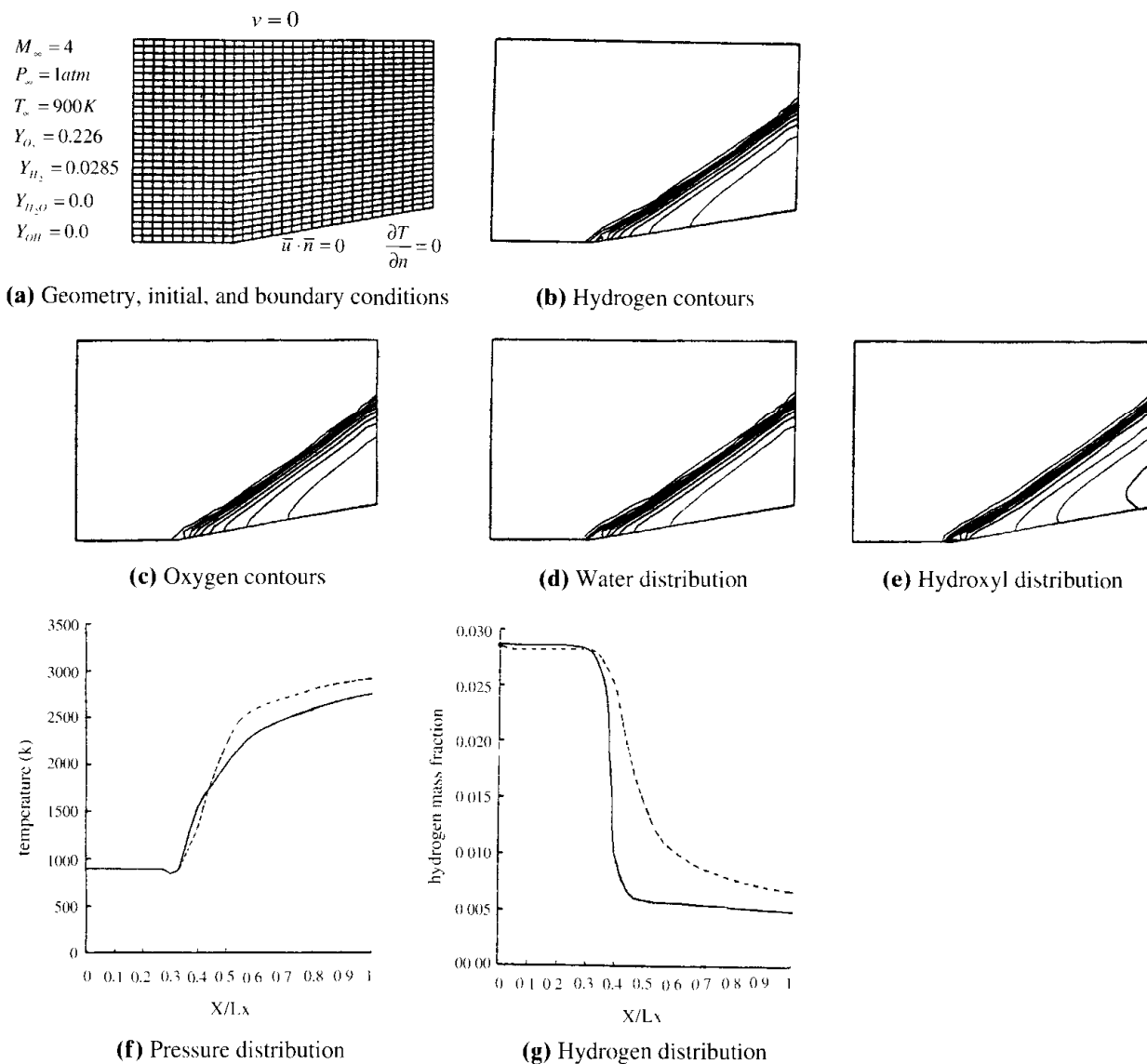
Figure 22.6.1.3 Ramjet combustion (hydrogen-air reactions), comparison of the result of 18-step with 2-step reactions [Yoon, 1992], — 18-step, ---- global 2-step.
