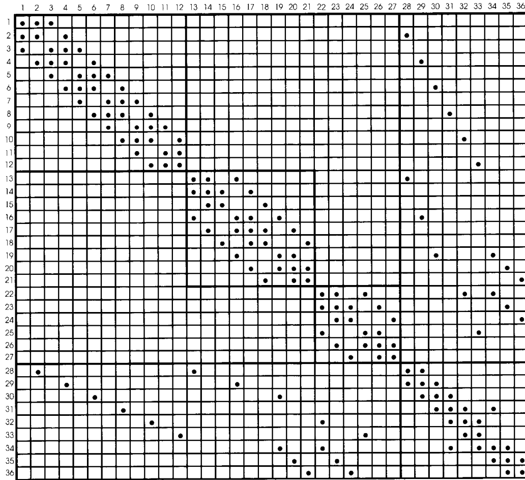
Figure 20.1.2 Global stiffness matrix, K_{aa}(27 \times 27) for Figure 20.2.1 with the subdomain stiffness matrices K_1(12 \times 12) , K_2(9 \times 9) , K_3(6 \times 6) , for \Omega_1 , \Omega_2 , \Omega_3 , respectively, and the boundary interface stiffness matrix, K_{bb}(9 \times 9) together with the interface-subdomain interaction stiffness matrices K_{ab}(27 \times 9) and K_{ba}(9 \times 27) .
