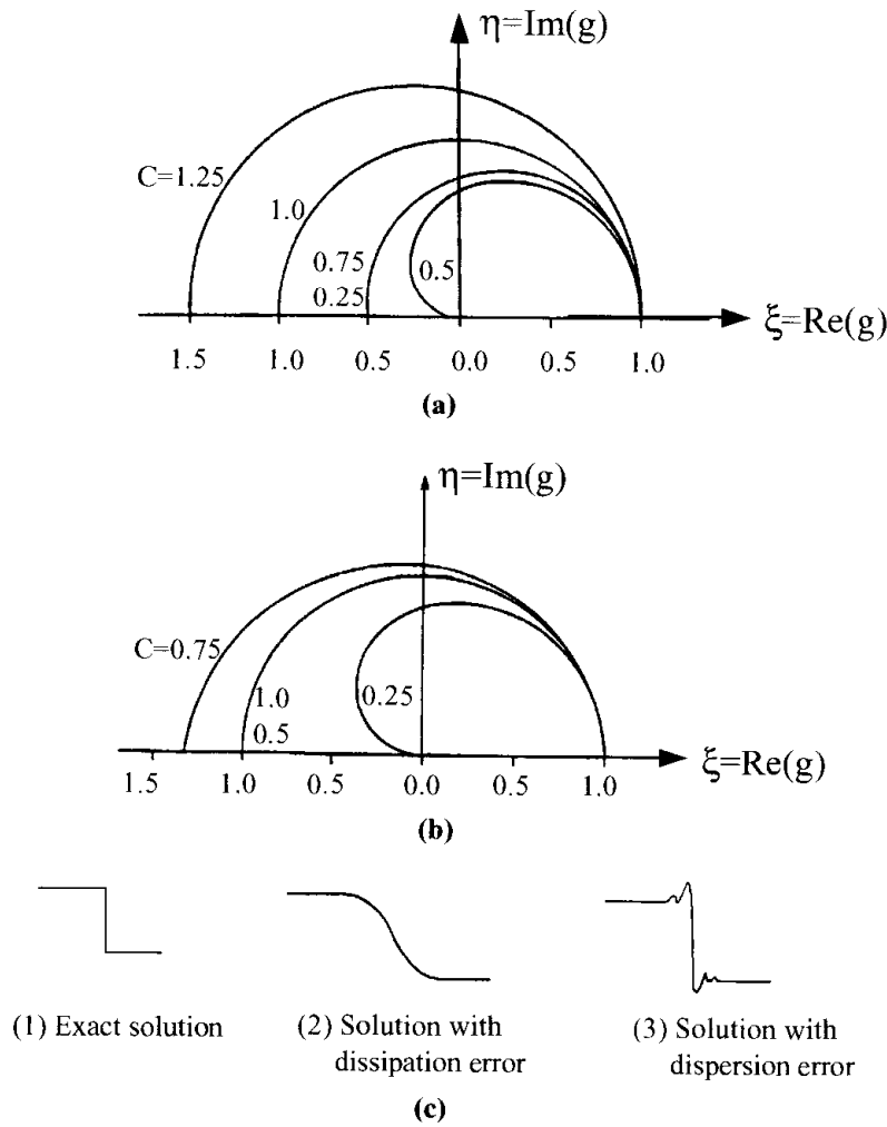
Figure 4.3.2 Dissipation and dispersion errors compared to exact solution. (a) Dissipation error (amplification factor modulus |g| ). (b) Dispersion error (relative phase error, \Phi/\tilde{\Phi} ). (c) Comparison of exact solution with dissipation error and dispersion error for shock tube problem.
