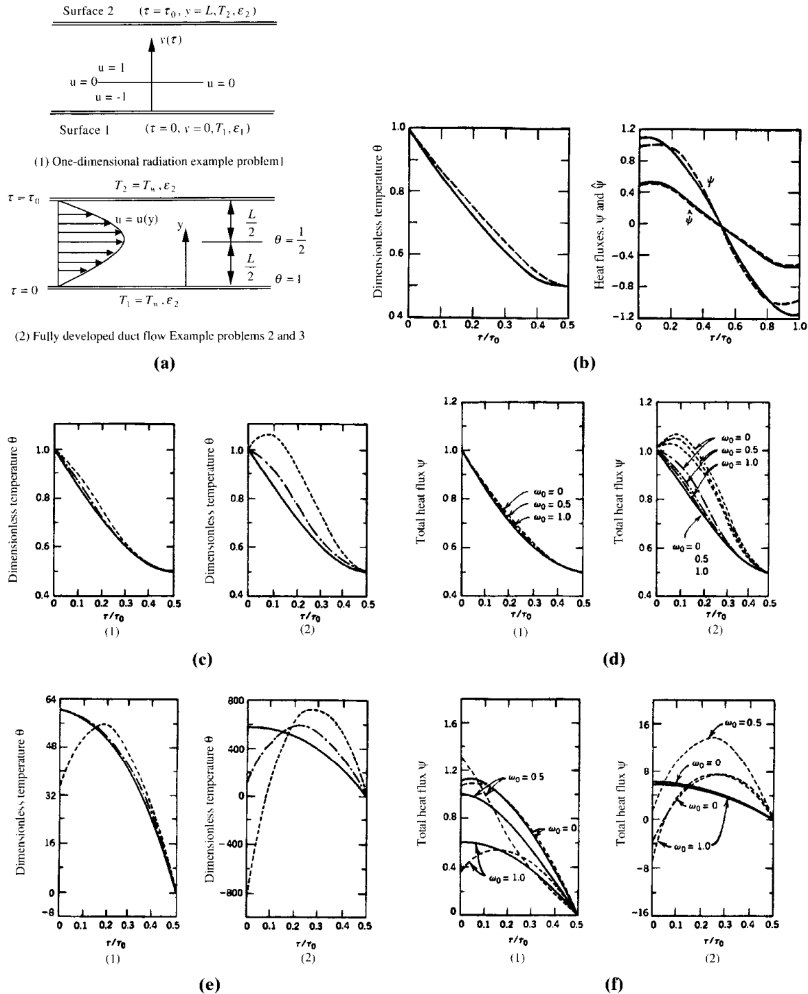
Figure 24.4.4.1 Combined mode conduction, convection, and radiation with and without scattering and viscous dissipation [Chung and Kim, 1984]. (a) Example problem. (1) One-dimensional radiation, example problem 1; (2) fully developed duct flow, example problems 2 and 3. (b) Combined conduction-convection-radiation heat transfer without scattering and viscous dissipation. N = 0.1 ; \omega_0 = 0 ; Ec Pr = 0 ; \tau_0 = \epsilon_1 = \epsilon_2 = 1 . (c) Combined conduction-convection-radiation heat transfer with scattering and viscous dissipation. N = 0.1 ; \epsilon_1 = \epsilon_2 = 1 . (1) \tau_0 = 1.0 ; (2) \tau_0 = 0.1 . (—) Ec Pr = 0 , \omega_0 = 1.0 ; (—•—) Ec Pr = 0.5 , \omega_0 = 0.5 ; (-----) Ec Pr = 1.0 , \omega_0 = 0 . (d) Combined conduction-convection-radiation heat transfer, with scattering and viscous dissipation. N = 0.1 ; \epsilon_1 = \epsilon_2 = 1 . (1) \tau_0 = 1.0 ; \tau_0 = 0.1 . (—) Ec Pr = 0 ; (—•—) Ec Pr = 0.5 ; (-----) Ec Pr = 1.0 . (e) Combined conduction-convection-radiation heat transfer (temperature distributions) with scattering and viscous dissipation. N = 0.1 ; \epsilon_1 = \epsilon_2 = 1 . (1) \tau_0 = 1.0 ; \tau_0 = 0.1 . (—) Ec Pr = 0 , \omega_0 = 1.0 ; (—•—) Ec Pr = 0.5 , \omega_0 = 0.5 ; (-----) Ec Pr = 1.0 , \omega_0 = 0 . (f) Combined conduction-convection-radiation heat transfer (heat flux distributions) with scattering and viscous dissipation. N = 0.1 ; \epsilon_1 = \epsilon_2 = 1 . (1) \tau_0 = 1.0 ; (2) \tau_0 = 0.1 . (—) Ec Pr = 0 ; (-----) Ec Pr = 1.0 .
