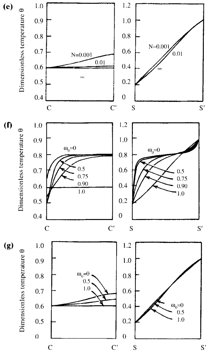
Figure 24.4.5.1 (continued.) (e) Effects of N on the temperature profiles along CC' and SS' . \tau_0 = 0.1 ; \omega_0 = 0 ; \text{Re Pr} = 100 . (f) Effects of albedo \omega_0 on the temperature profiles along CC' and SS' . \tau_0 = 1.0 ; N = 0.00 ; \text{Re Pr} = 100 . (g) Effects of albedo \omega_0 on the temperature profiles along CC' and SS' . \tau_0 = 0.1 ; N = 0.00 ; \text{Re Pr} = 100 .
