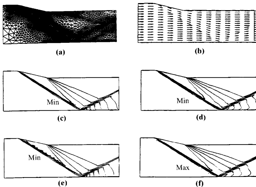
Figure 19.2.3 Mesh refinements ( h -method), triangular elements. (a) Adapted mesh configuration (5004 elements, 2600 nodes, t = 0.059 sec). (b) Velocity field (Inlet vel. = 1506 m/sec). (c) Density contours (Max = 1.648, Min = 0.418, \Delta = 0.123 kg/m 3 ). (d) Temperature contours (Max = 1588, Min = 863, \Delta = 73 K). (e) Pressure contours (Max = 0.725, Min = 0.115, \Delta = 0.061 MPa). (f) Mach number contours (Max = 2.603, Min = 1.152, \Delta = 0.145 ).
