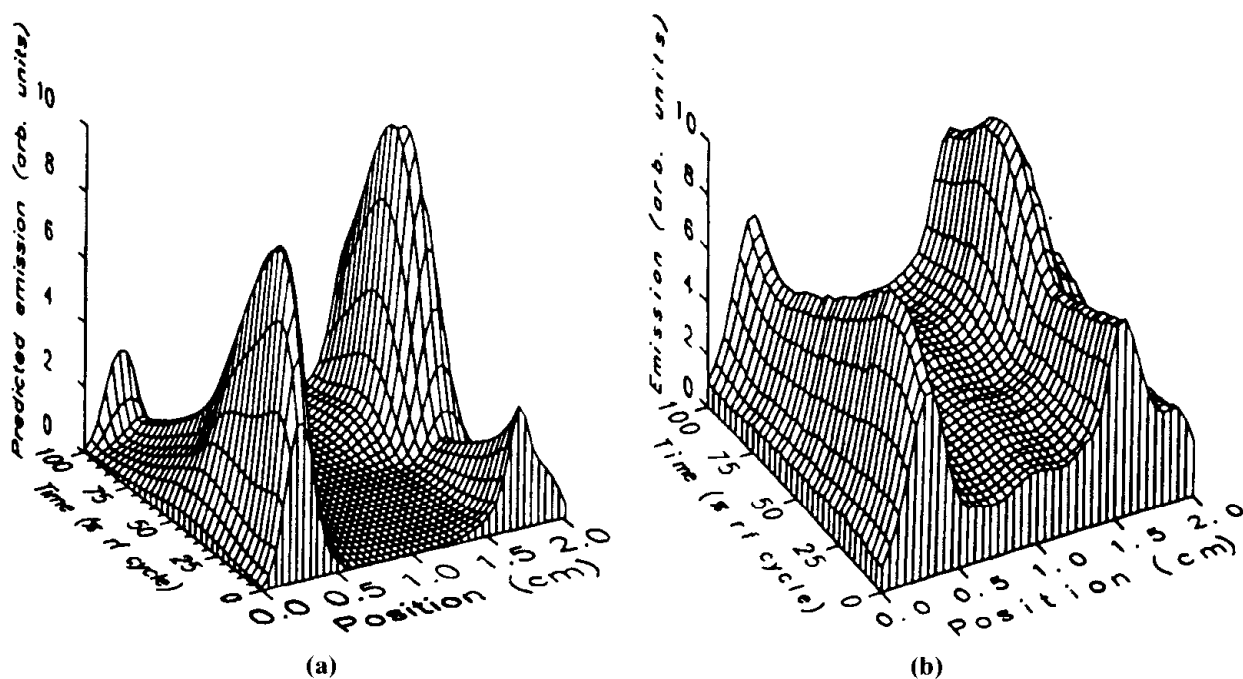
Figure 26.4.2.1 RF glow discharge [Gogolides and Swain, 1992]. (a) Predictions from a two-moment model for emission of the 750.4-nm argon line (1 torr, 2 cm spacing, 13.5 Mhz, and 0.14 \text{ W/cm}^2 ). (b) Experimentally measured emission.
