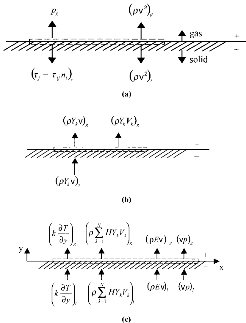
Figure 22.2.1 Neumann boundary conditions for burning of solid fuel. (a) Momentum flux Neumann boundary conditions (Burning of solid fuel). (b) Species mass flux Neumann boundary conditions (Burning of solid fuel). (c) Energy flux Neumann boundary conditions (gas-liquid interface).
