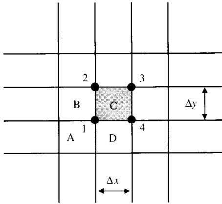
Figure 7.2.3 Cell-centered average scheme.
