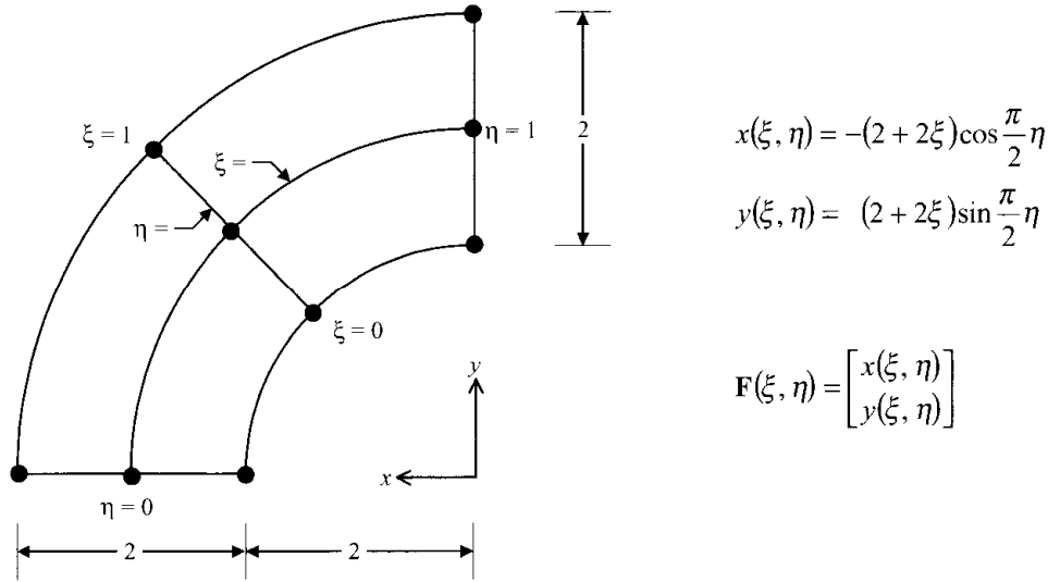
Figure E17.1.6 Quarter-circle disk with TIF method.
