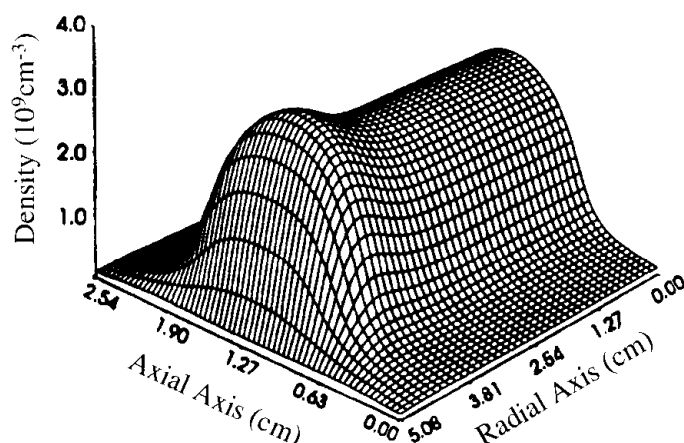
Figure 26.4.2.2 Two-dimensional profile of electron density in an argon discharge [Young and Wu, 1993].
