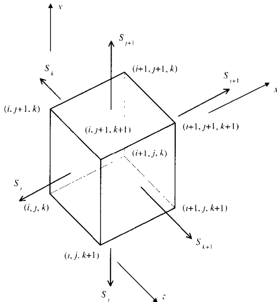
Figure 7.3.6 Three-dimensional discretization.
