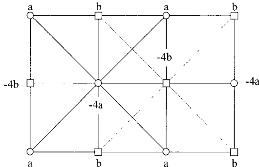
Figure 3.4.3 Odd-even oscillations of the five-point scheme.
