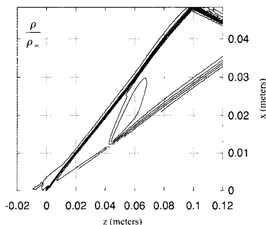
Figure 6.8.2.4 Inviscid fin shock interaction.
