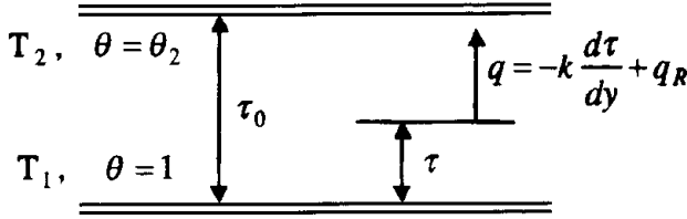
Figure 24.3.1 One-dimensional combined conduction and radiation.
