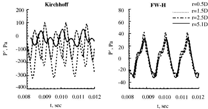
Figure 23.5.2.2 Acoustic signals computed for various integration surfaces [Singer et al., 1999].
