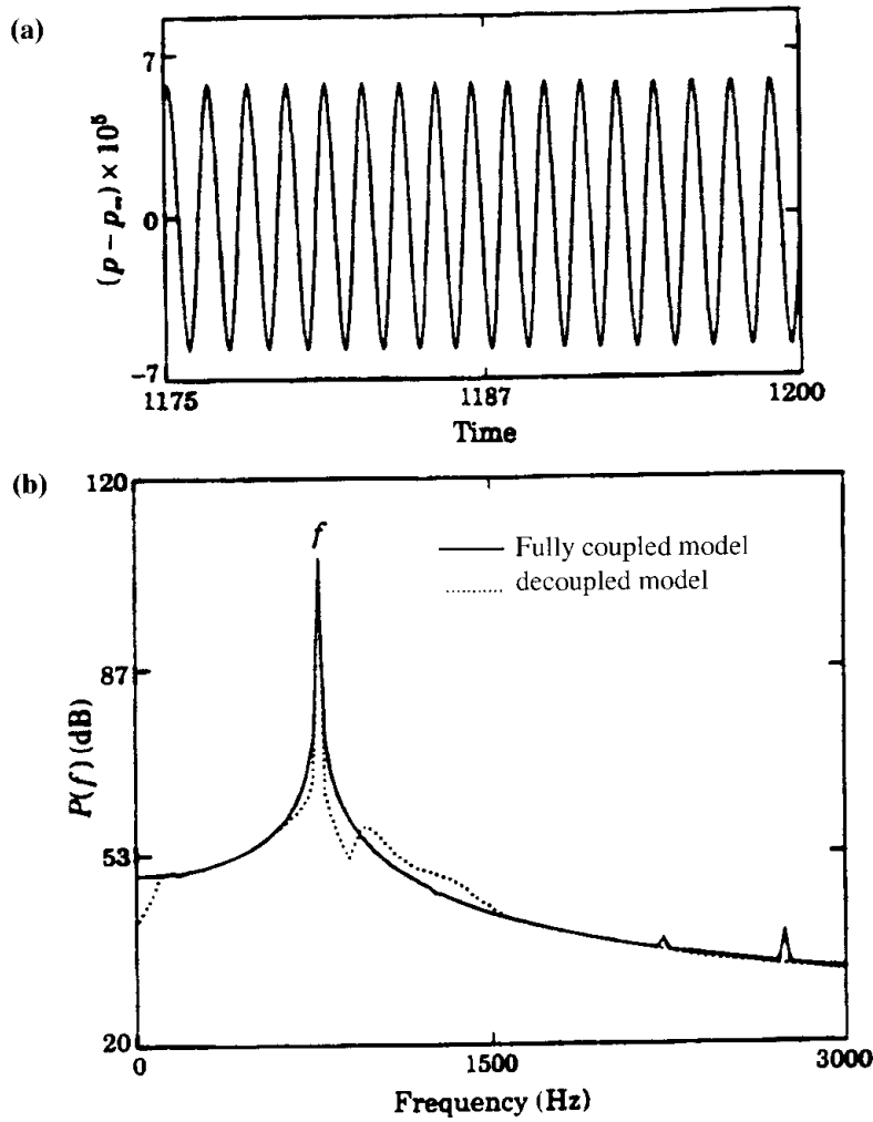
Figure 23.5.1.2 (a) The time history and (b) power spectral density of the transmitted near-field pressure, 2.54 cm from the panel center, for an excitation amplitude 130 dB (linear) [Frederi et al., 1995]. Reprinted with permission from Academic Press.
