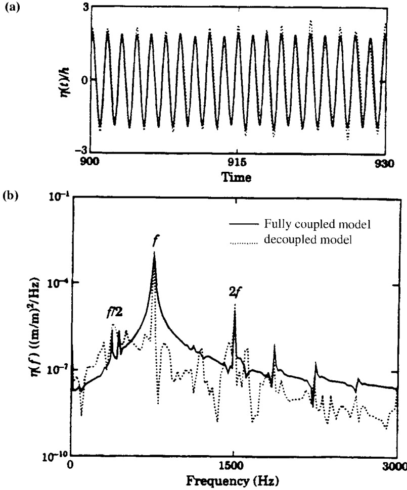
Figure 23.5.1.3 (a) The time history and (b) power spectral density of the panel center displacement for an excitation amplitude 174 dB (nonlinear) [Frendi et al., 1995]. Reprinted with permission from Academic Press.
