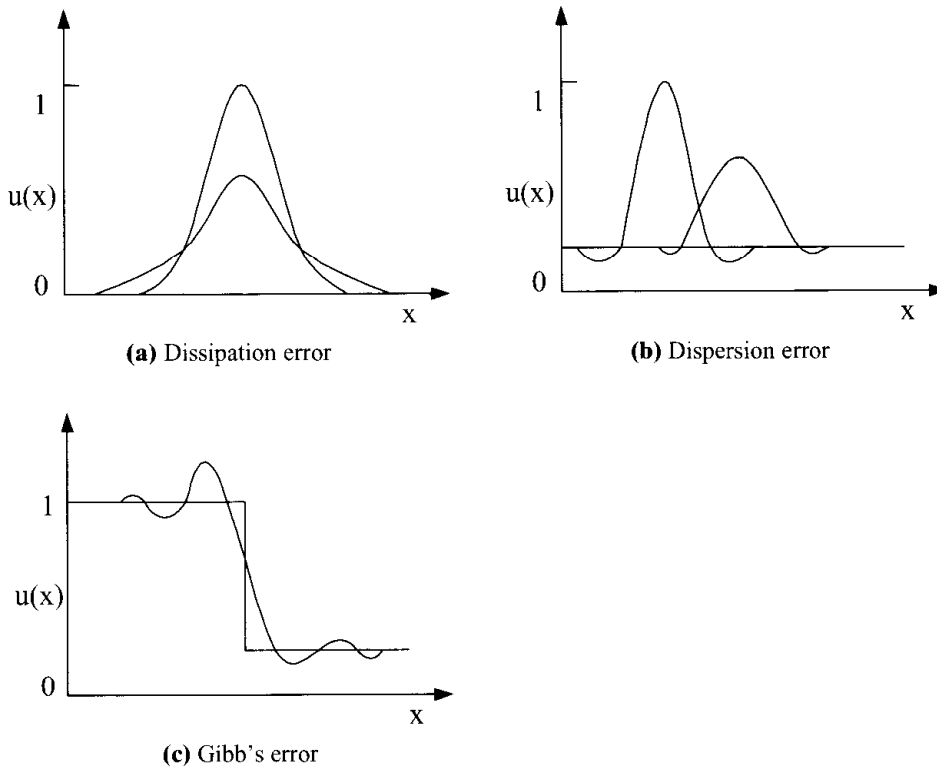
Figure 4.5.1 Various numerical errors.
