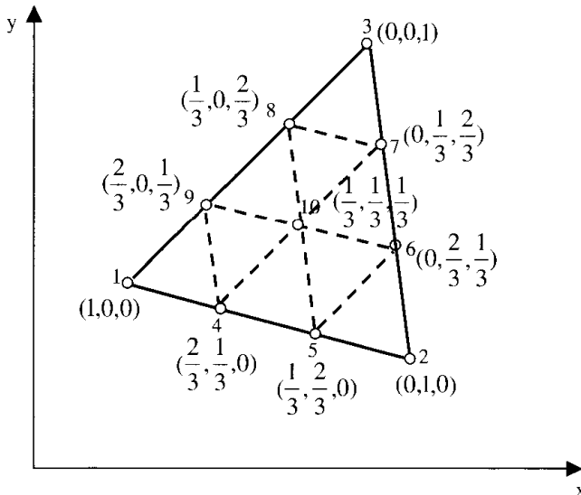
Figure 9.3.5 Natural coordinate triangular element (cubic variation).
