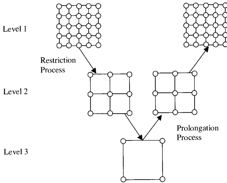
Figure 20.2.1 Three-level multigrid discretization.
