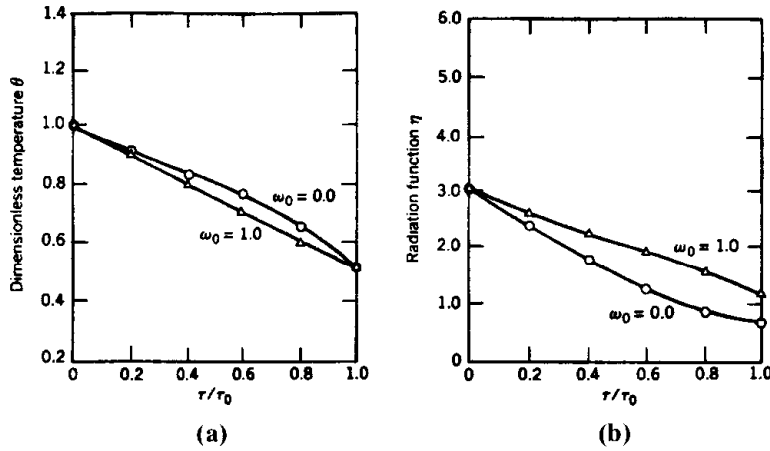
Figure 24.4.3.1 Combined conduction-radiation heat transfer, effects of \omega_0 on the temperature and radiation function for N = 1 , \tau_0 = \varepsilon_1 = \varepsilon_2 = 1.0 .
