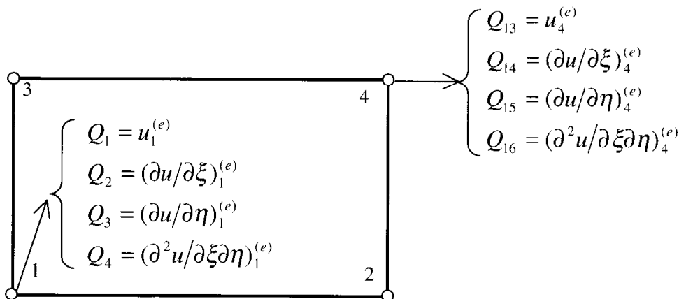
Figure 9.3.9 Hermite bicubic rectangular element.
