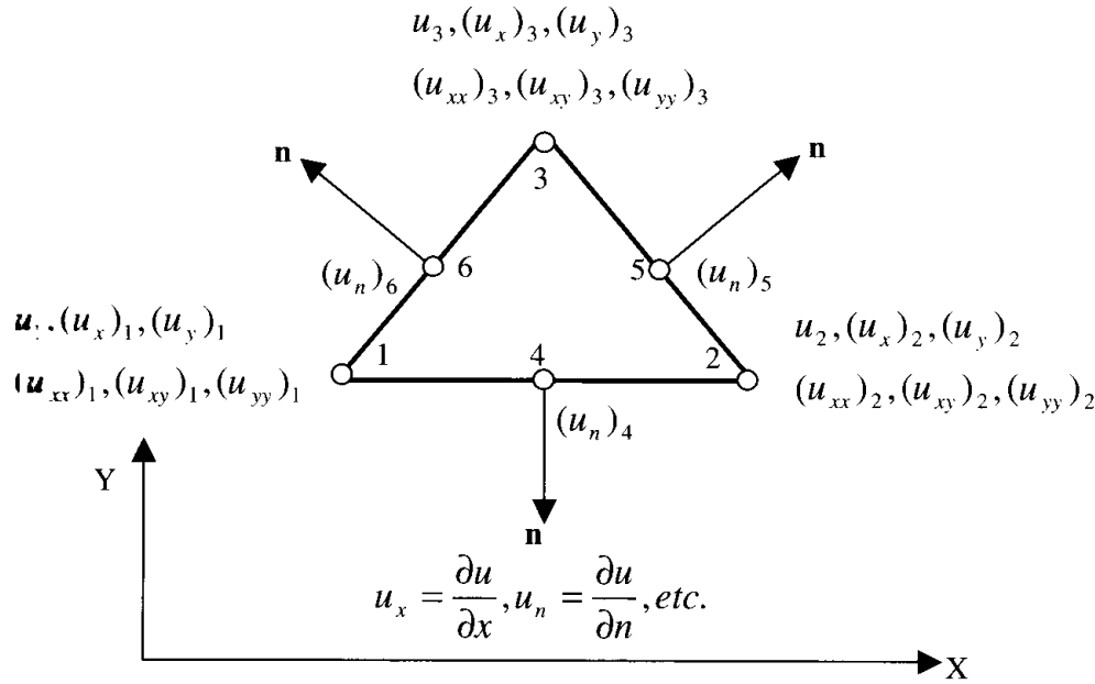
Figure 9.6.1 Hermite triangle, 21 constants to be determined.
