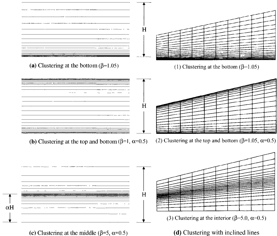
Figure E17.1.4 Clustering of mesh lines.
