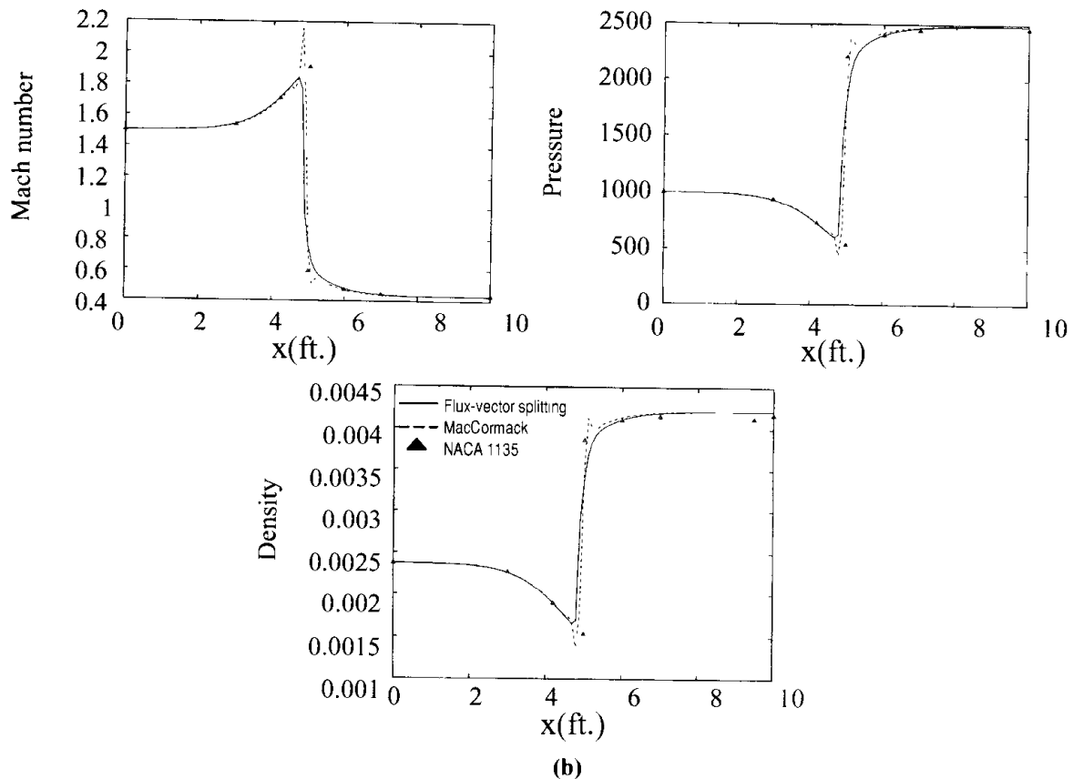
Figure 6.8.1.1 Quasi-one-dimensional supersonic nozzle flow. (a) Case 1 supersonic inflow-supersonic outflow. (b) Case 2 supersonic inflow-supersonic outflow.
