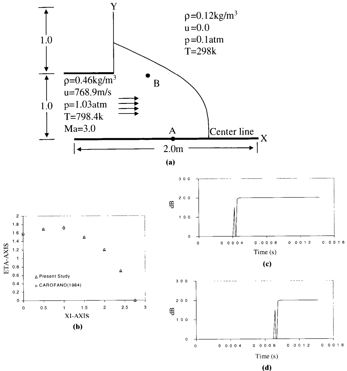
Figure 23.5.1.10 Geometry, initial and boundary conditions for the rocket nozzle exhaust. (a) Geometry and initial and boundary condition. (b) Shock locations at t = 0.0012 \text{ sec} . (c) Noise level at point A. (d) Noise level at point B.
