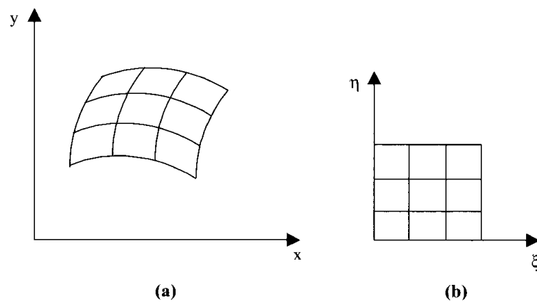
Figure 4.6.1 Transformation from curvilinear grid system into rectangular grid system. (a) Original curvilinear grid. (b) Transformed cartesian grid.
