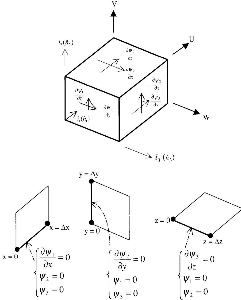
Figure 12.2.2 Three-dimensional boundary conditions.
