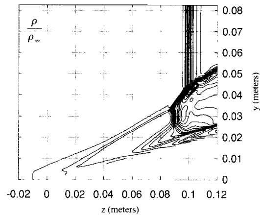
Figure 6.8.2.6 Boundary layer separation on the ramp.
