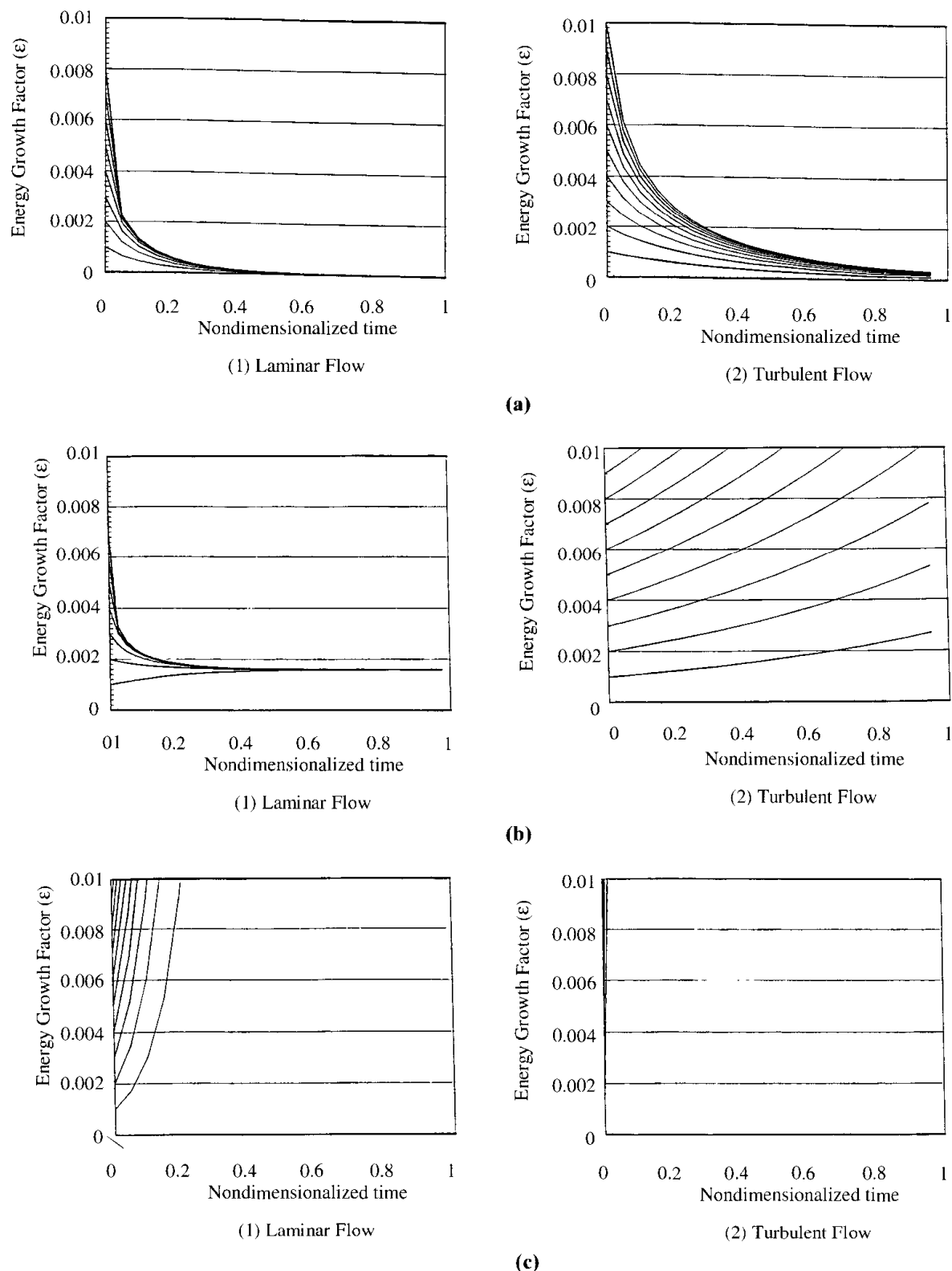
Figure 23.5.3.2 Energy growth factors vs. nondimensionalized time [Yoon and Chung, 1994]. (a) 4% disturbance. (b) 6% disturbance. (c) 8% disturbance.
