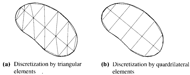
Figure 9.1.1 Finite element discretization of a two-dimensional domain.
