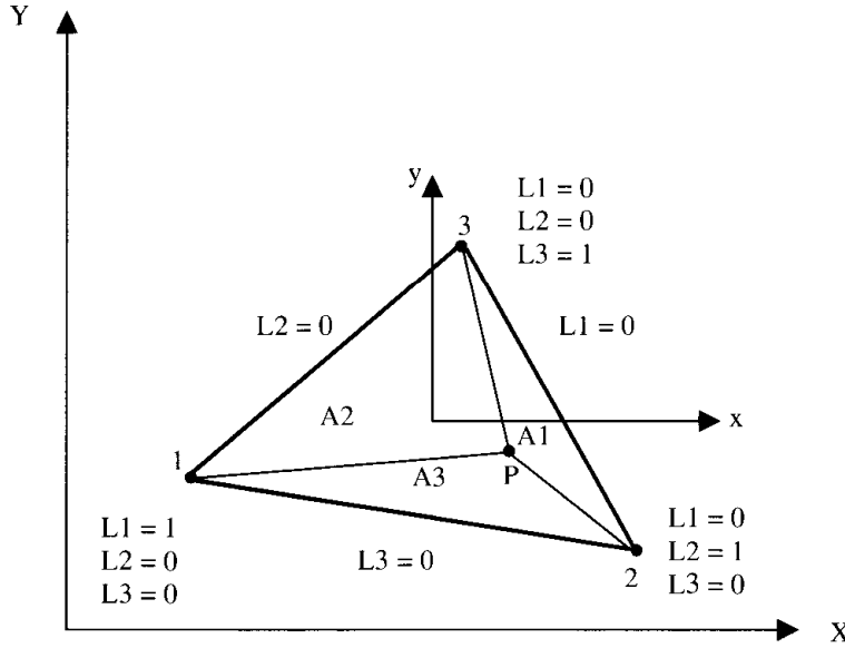
Figure 9.3.3 Natural coordinate triangular element (linear variation).
