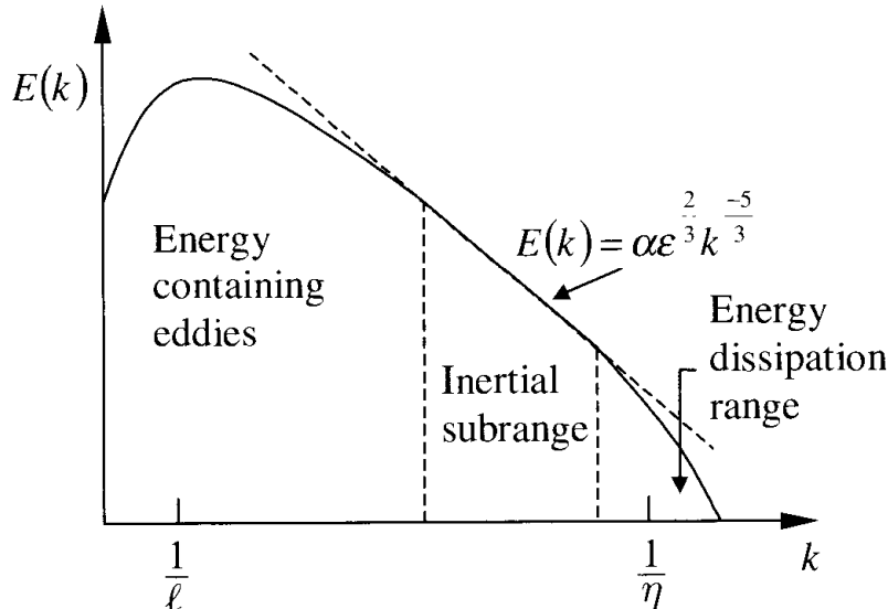
Figure 21.4.1 Energy spectrum vs. wave number space (log-log scales).
