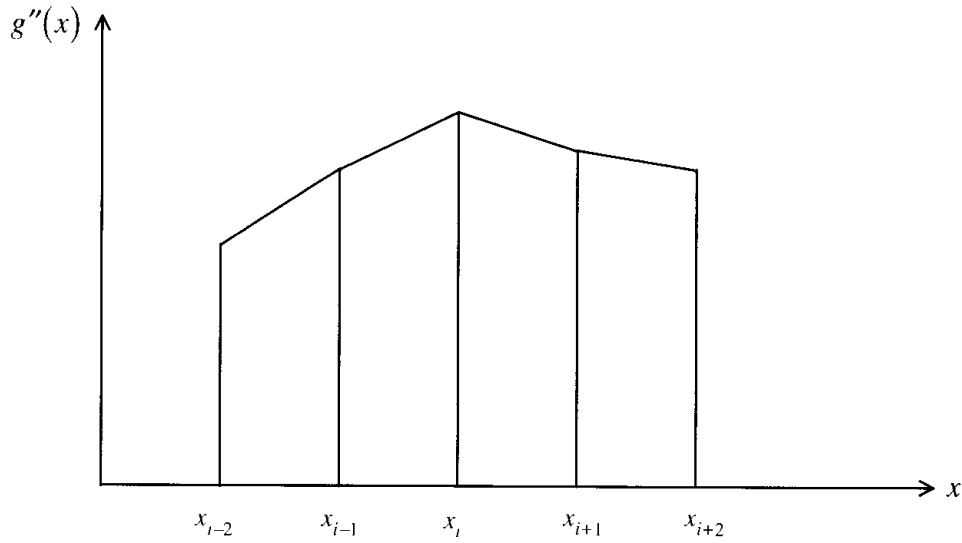
Figure 17.1.3 Cubic spline representation.
