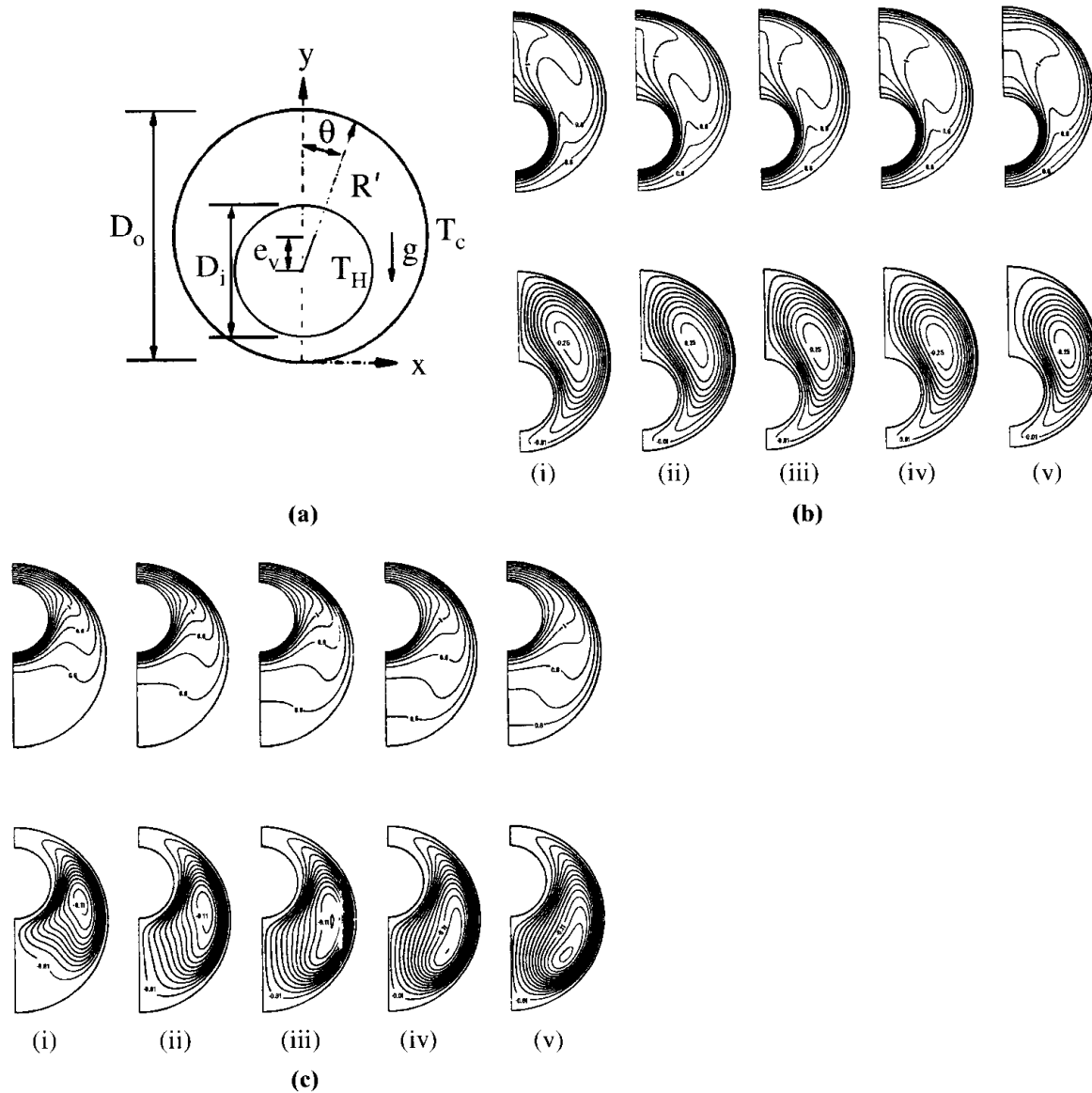
Figure 24.4.4.2 Effects of radiation on natural convection [Han and Baek, 1999]. (a) Eccentric annular cross section. (b) Isotherms (upper, \Delta T = 0.1 ) and streamlines (lower, \Delta \psi = 0.03 ) in an eccentric annulus ( e_v/L = 0.623 ) for various conduction to radiation parameters N with Ra = 1.5 \times 10^4 , \delta = 1 , \tau_0 = 0.3 , \omega_0 = 0 , and black boundaries: (i) without radiation, (ii) N = 0.1 , (iii) N = 0.05 , (iv) N = 0.03 , and (v) N = 0.02 . (c) Isotherms (upper, \Delta T = 0.1 ) and streamlines (lower, \Delta \psi = 0.03 ) in an eccentric annulus ( e_v/L = -0.623 ) for various conduction to radiation parameters N with Ra = 1.5 \times 10^4 , \delta = 1 , \tau_0 = 0.3 , \omega_0 = 0 , and black boundaries: (i) without radiation, (ii) N = 0.1 , (iii) N = 0.05 , (iv) N = 0.03 , and (v) N = 0.02 .
