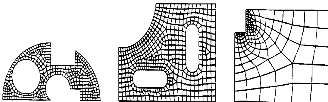
Figure 18.5.3 Examples of paving method [Blacker and Stephenson, 1991].
