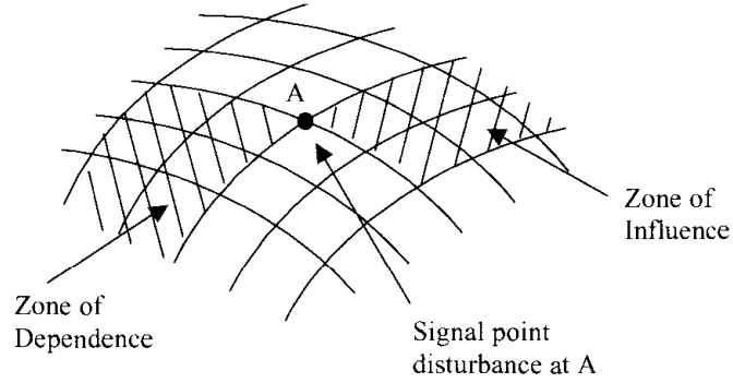
Figure 2.1.2 Propagation of disturbance and characteristics.
