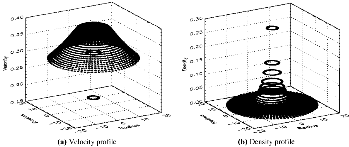
Figure 27.3.4.3 Dust infall velocity and density profiles [Richardson, 2000].
