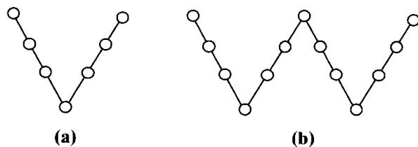
Figure 20.2.3 (a) V-cycle multigrid. (b) W-cycle multigrid.
