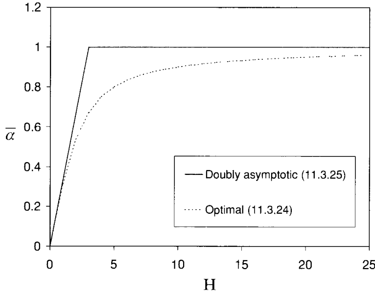
Figure 11.3.2 Effective numerical diffusivity \bar{\alpha} .
