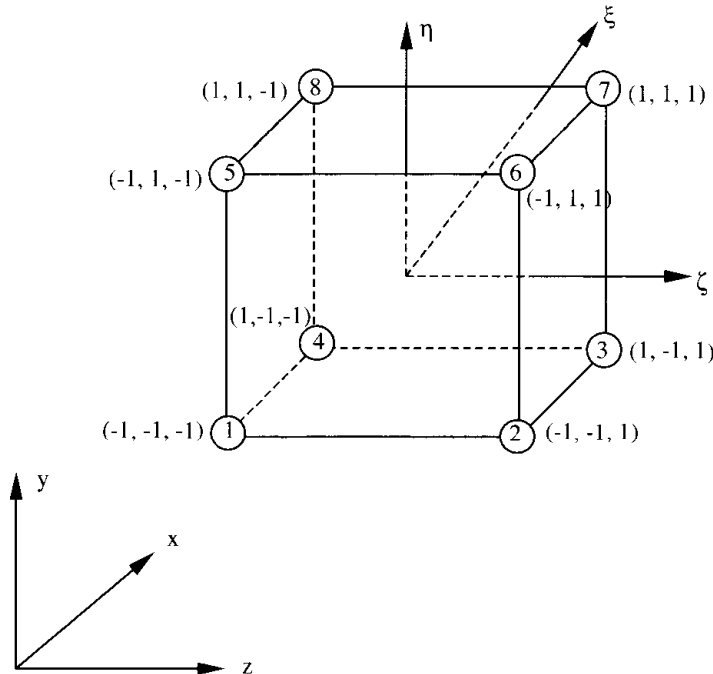
Figure 12.2.1 Hexahedral element for 3-D vortex transport analysis.
