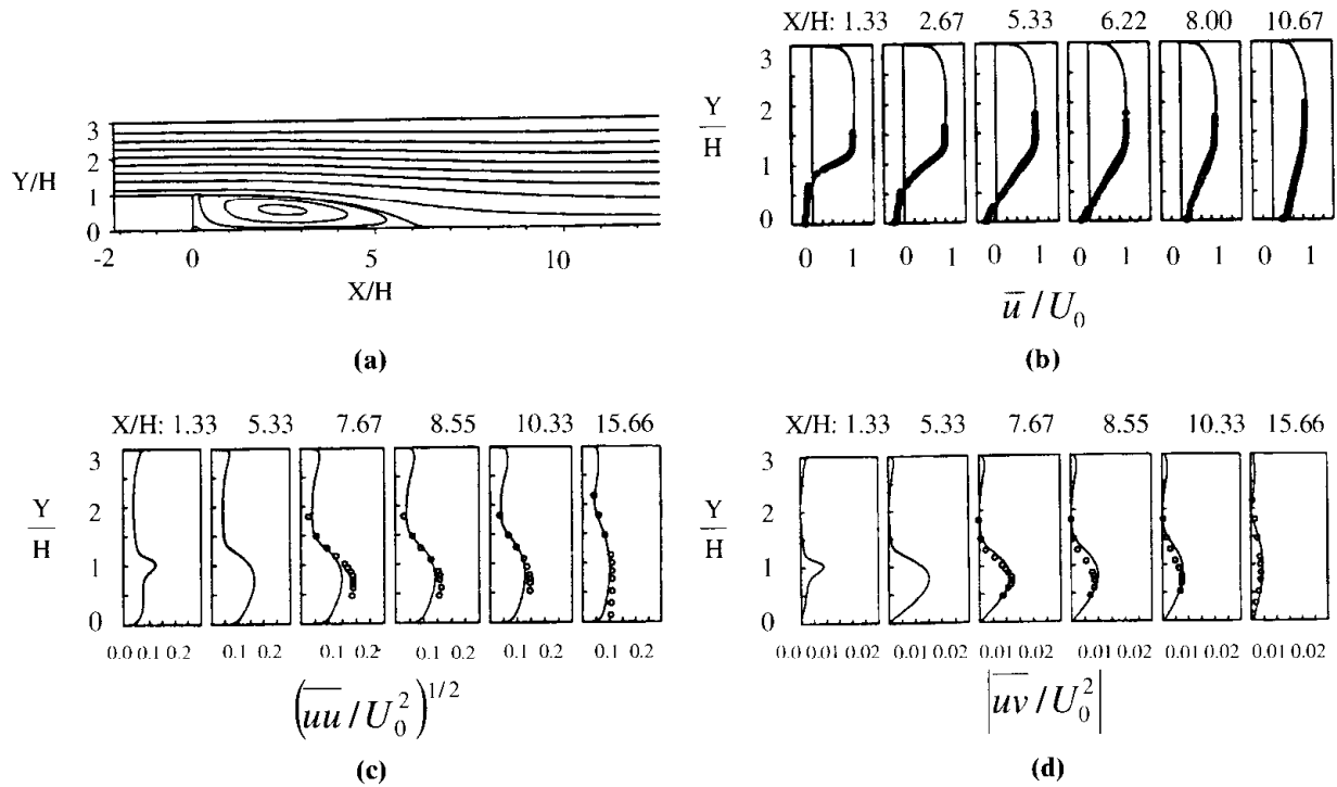
Figure 21.7.1.3 Results with the standard K-ε three-layer model [Thangam and Speziale, 1988]. (a) Contours of mean streamlines. (b) Mean velocity profiles at selected locations, compared with experiments [Kim et al., 1980]. (c) Turbulence intensity profiles. (d) Turbulence shear stress profiles.
