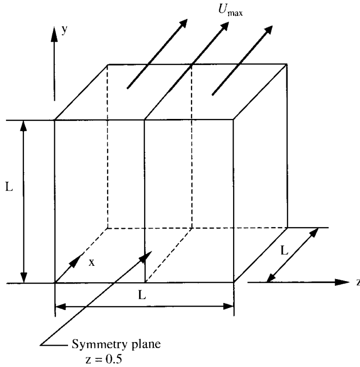
Figure 12.3.1 Geometry of the cubic cavity flow.
