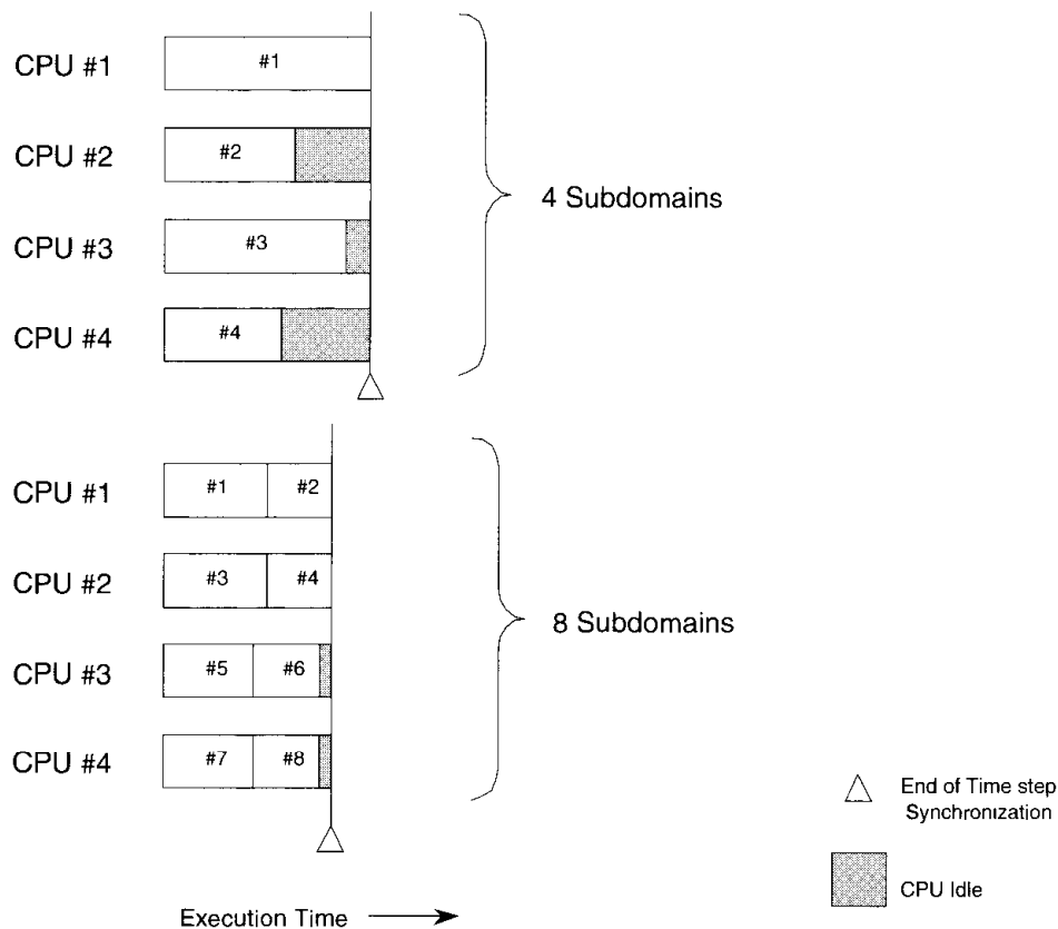
Figure 20.4.2.5 Domain decomposition improves parallelism.
