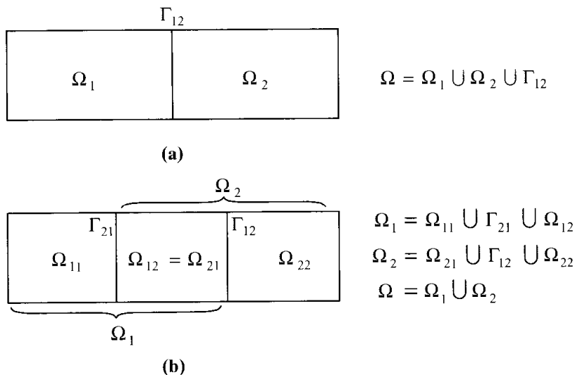
Figure 20.4.1 Domain decomposition. (a) Nonoverlapping subdomains. (b) Overlapping subdomains.
