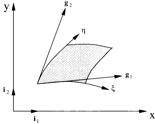
Figure 9.3.13 Coordinate transformation.
