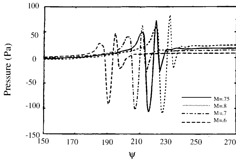
Figure 23.5.1.8 Different Mach numbers for hover parallel BVI, M = 0.8, 0.75, 0.7 , and 0.6 , \Gamma_v = 0.2 , Z_v = -0.26 at position d = 3R , \alpha = 60^\circ , \beta = -30^\circ [Xue and Lyrintzis, 1994].
