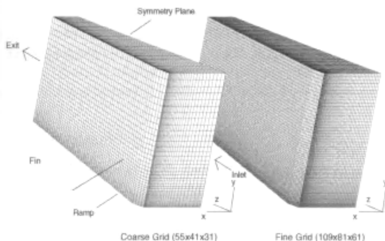
Figure 6.8.2.3 Three-dimensional finite difference models.
